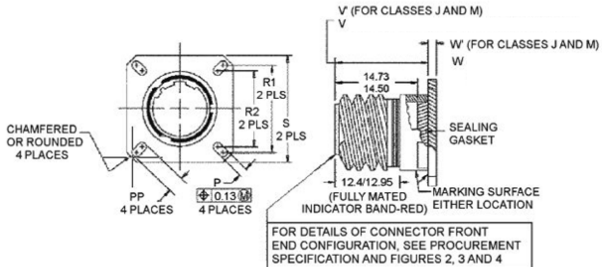
FIGURE 1. Dummy stowage receptacle.
