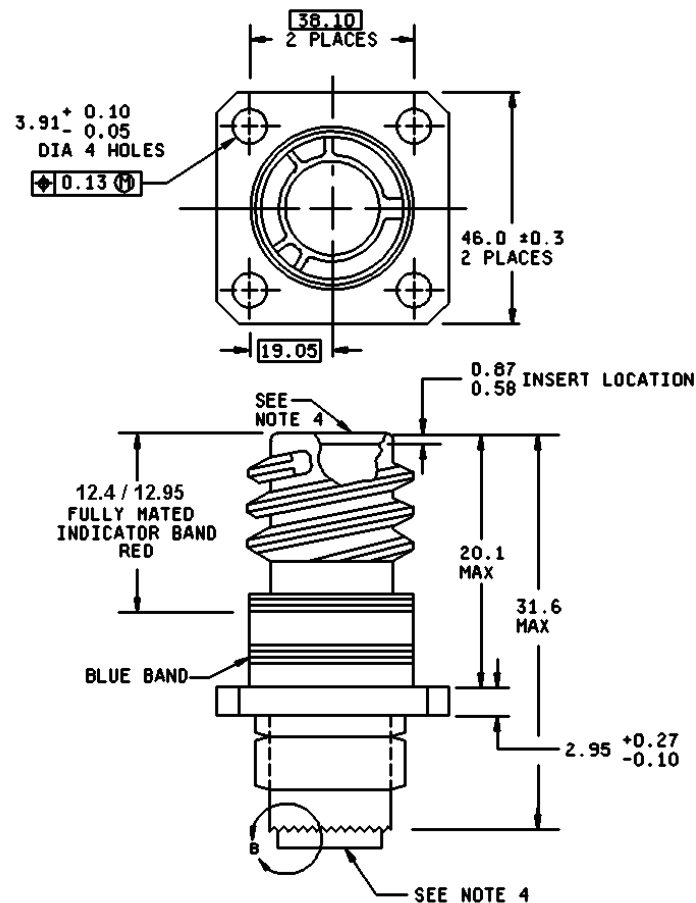
FIGURE 1. Receptacle, classes J, M, R, T, W and Z.
