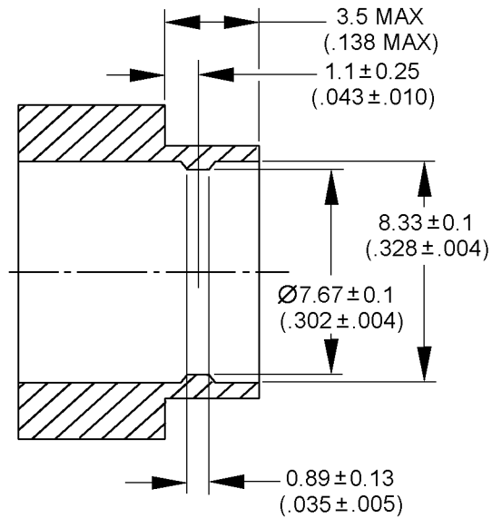
FIGURE 2. Recommended grommet cavity dimensions, sealing boot, size 8, shielded crimp contacts, configuration.
