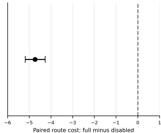
Figure A1. Supplementary paired route-cost comparison for the 300 held-out seeds. The locked estimate is full minus route-disabled = -4.737 units (95% bootstrap CI -5.186 to -4.268); completion did not change.
