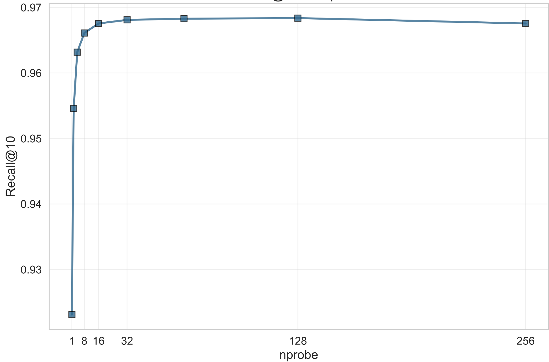
Recall@10 vs nprobe
