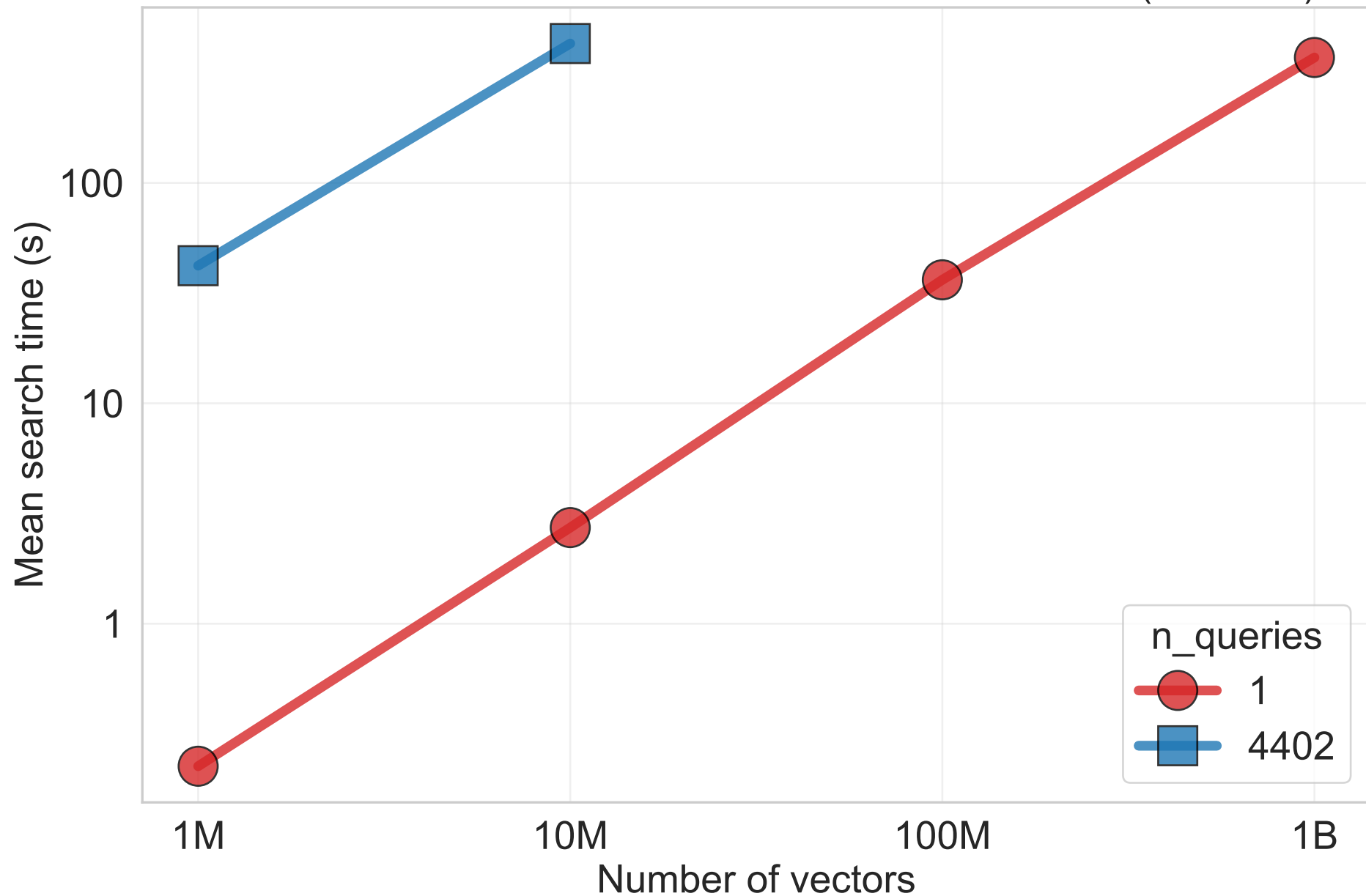
Exact search: mean search time vs number of vectors (k = 1000)
