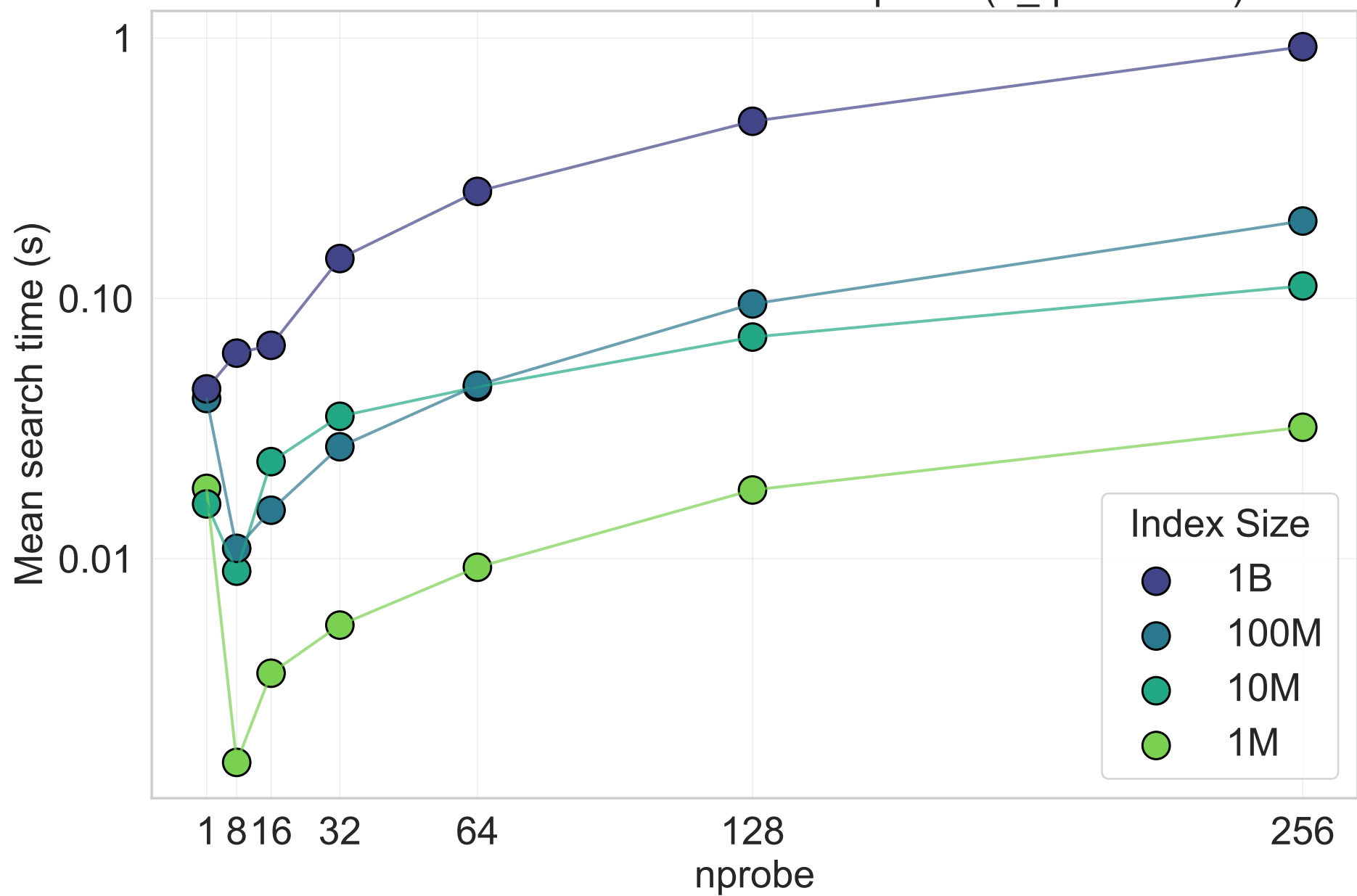
IVF search: mean search time vs. nprobe (n_queries = 1)
