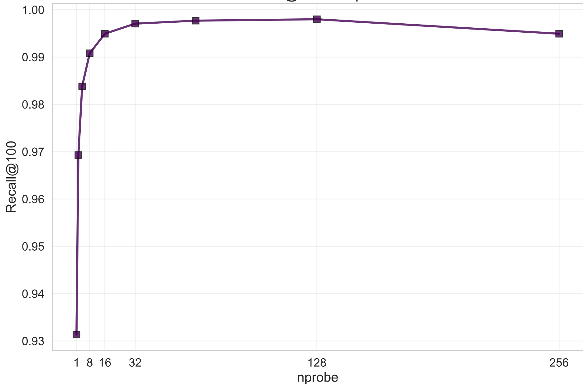
Recall@100 vs nprobe
