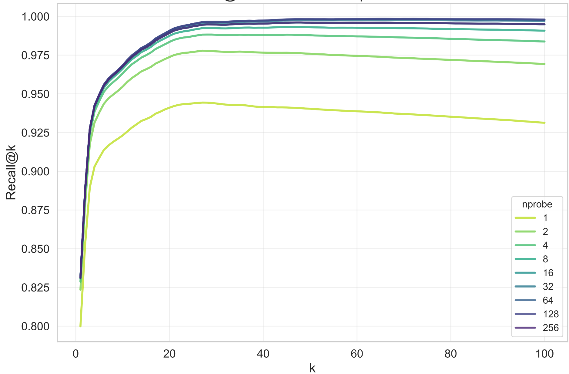
Recall@k across different nprobe values
