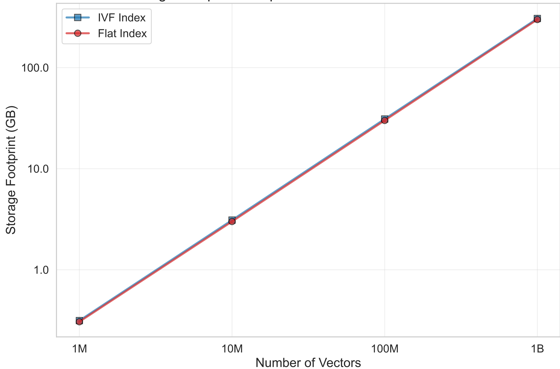
Storage Footprint Comparison: IVF vs Flat Search Indices
