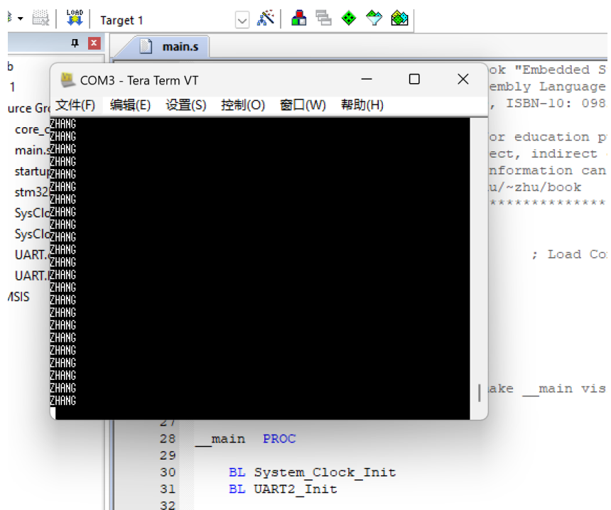
Figure 2: Display result of Stefan Zhang’s surname in Tera Term.
