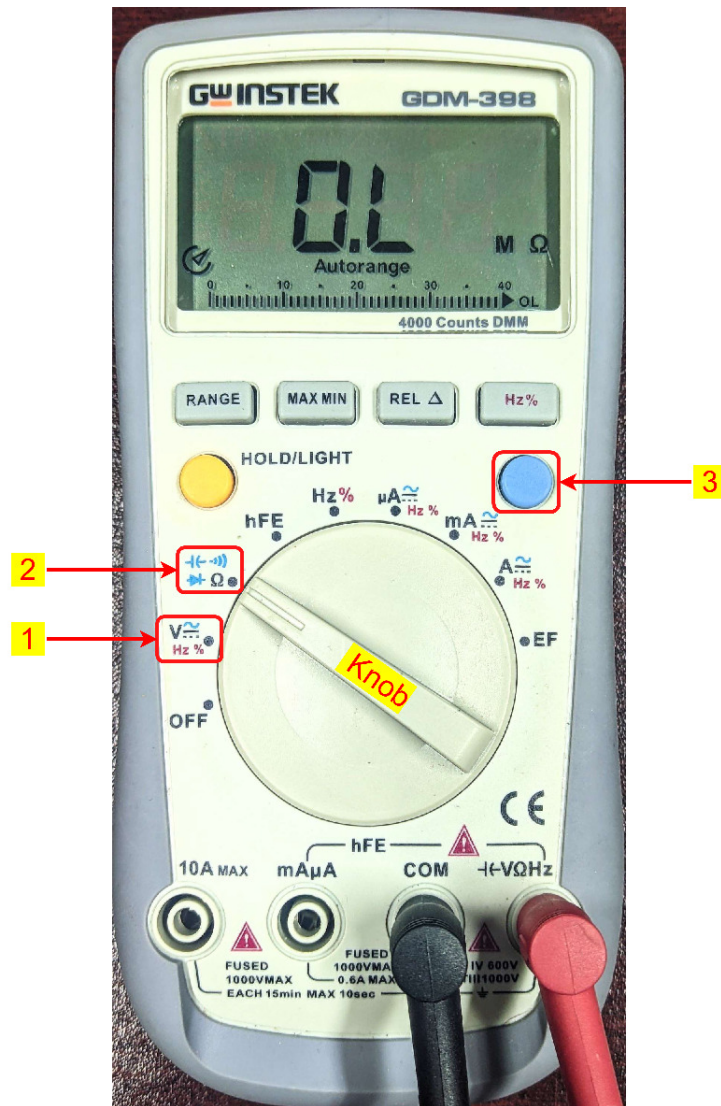
Figure 3: Digital Multimeter
