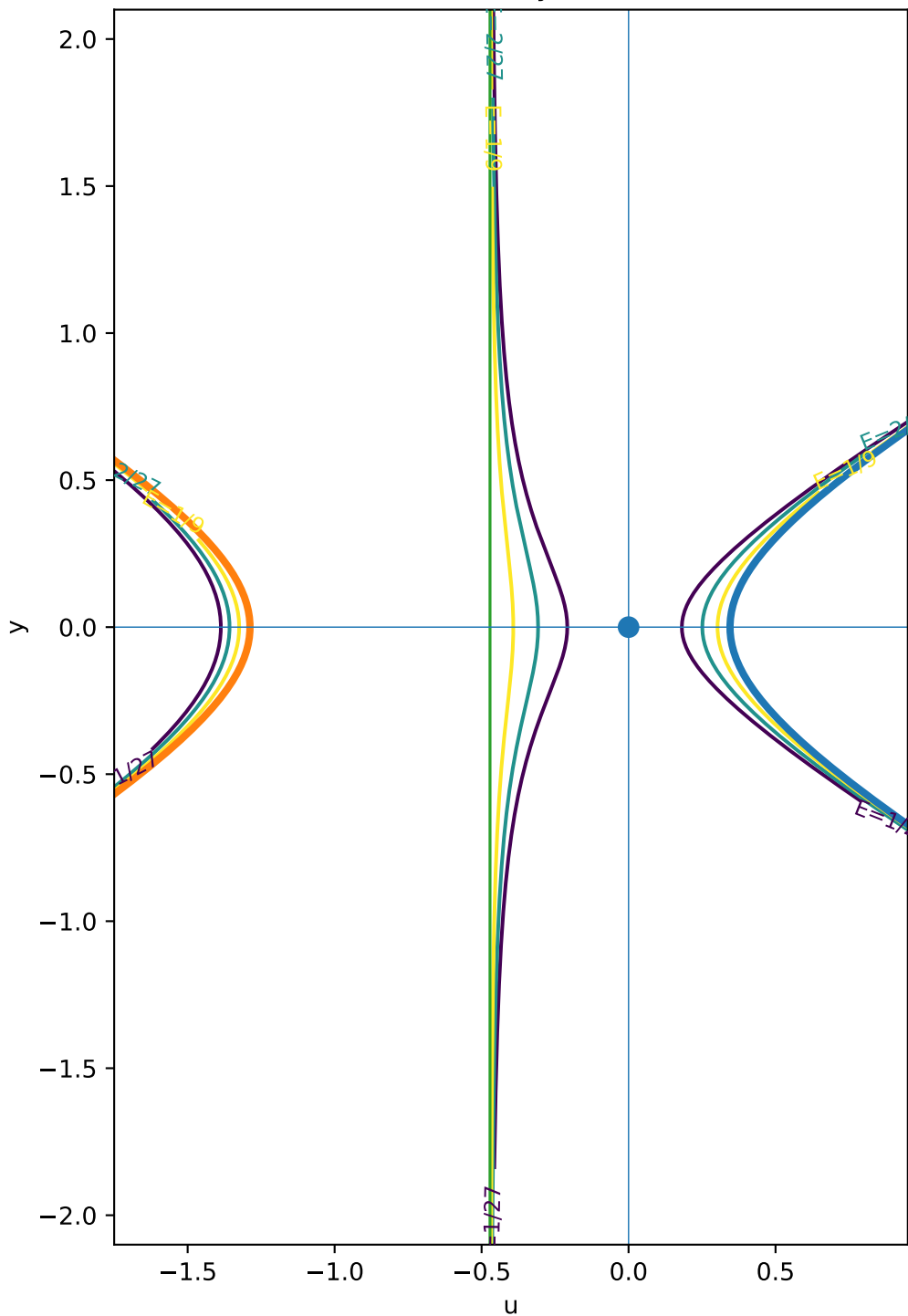
Abel-Wick traces v \rightarrow i y from the E=0 disk
