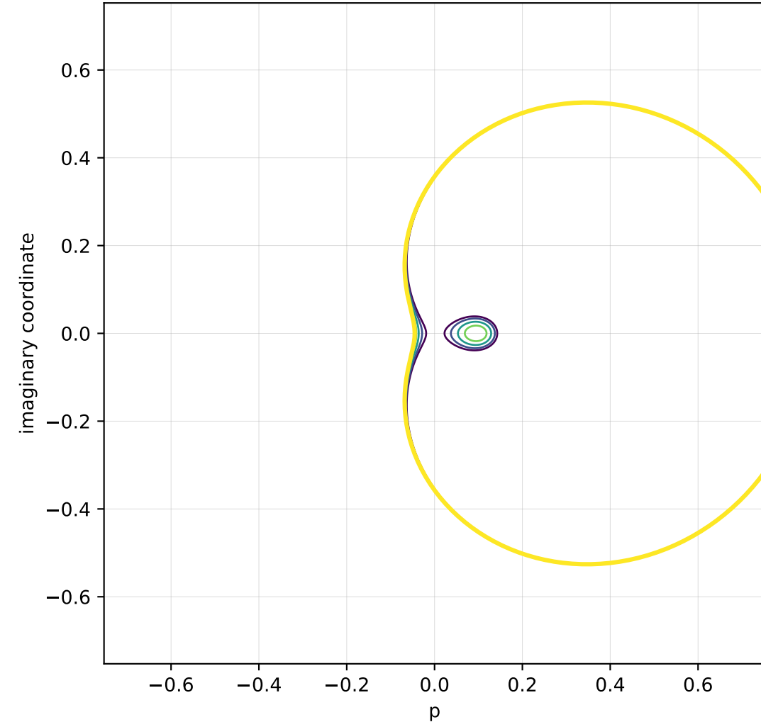
Abel-Wick real trace ( q \rightarrow iq )
