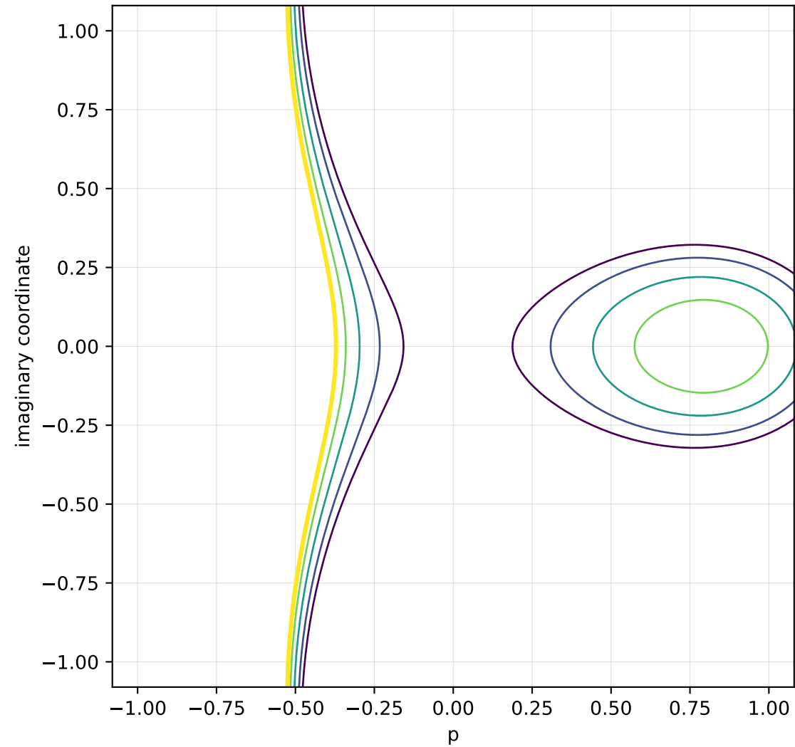
Abel-Wick real trace ( q \rightarrow iq )
