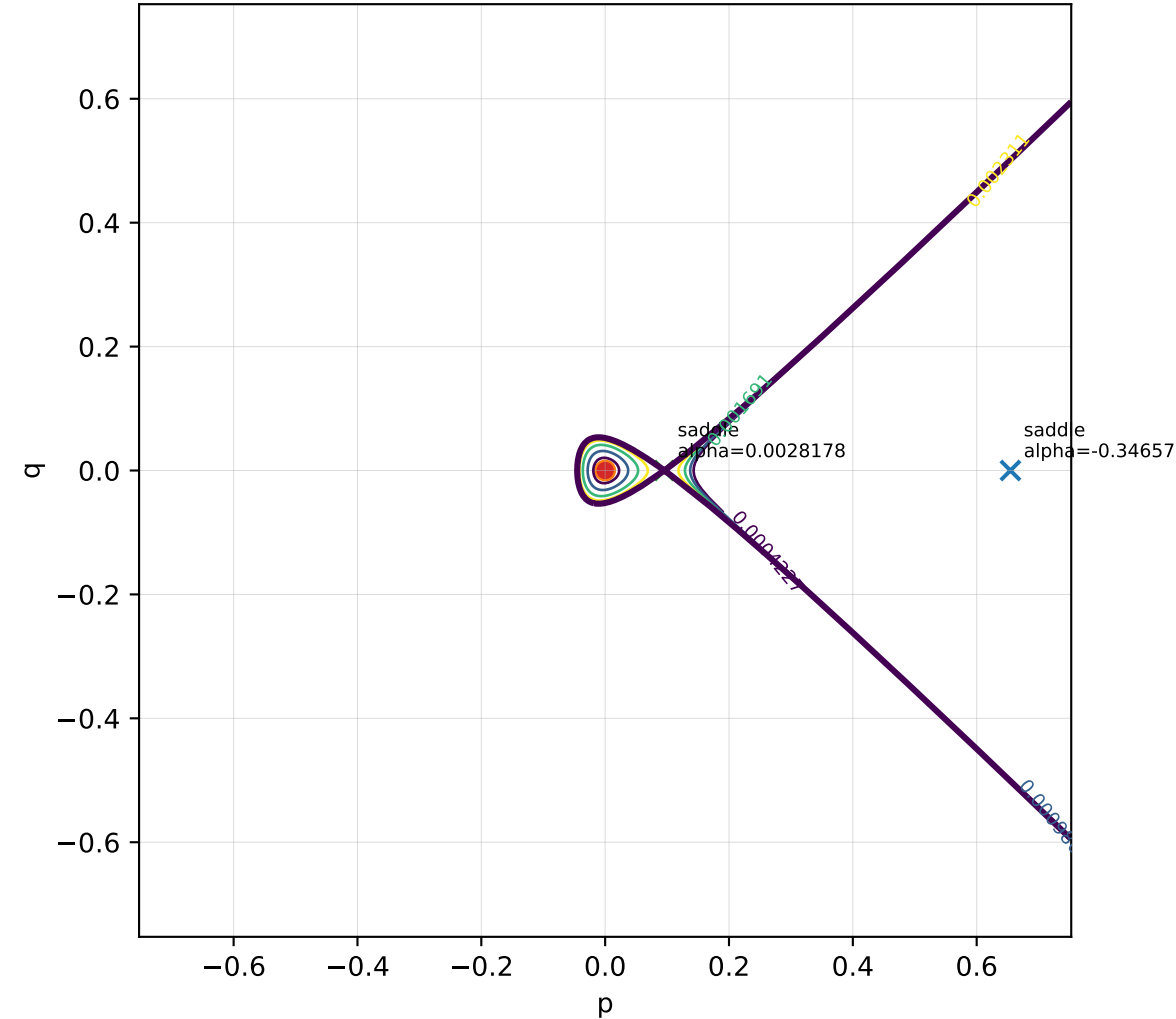
Real oscillation disk and critical level
