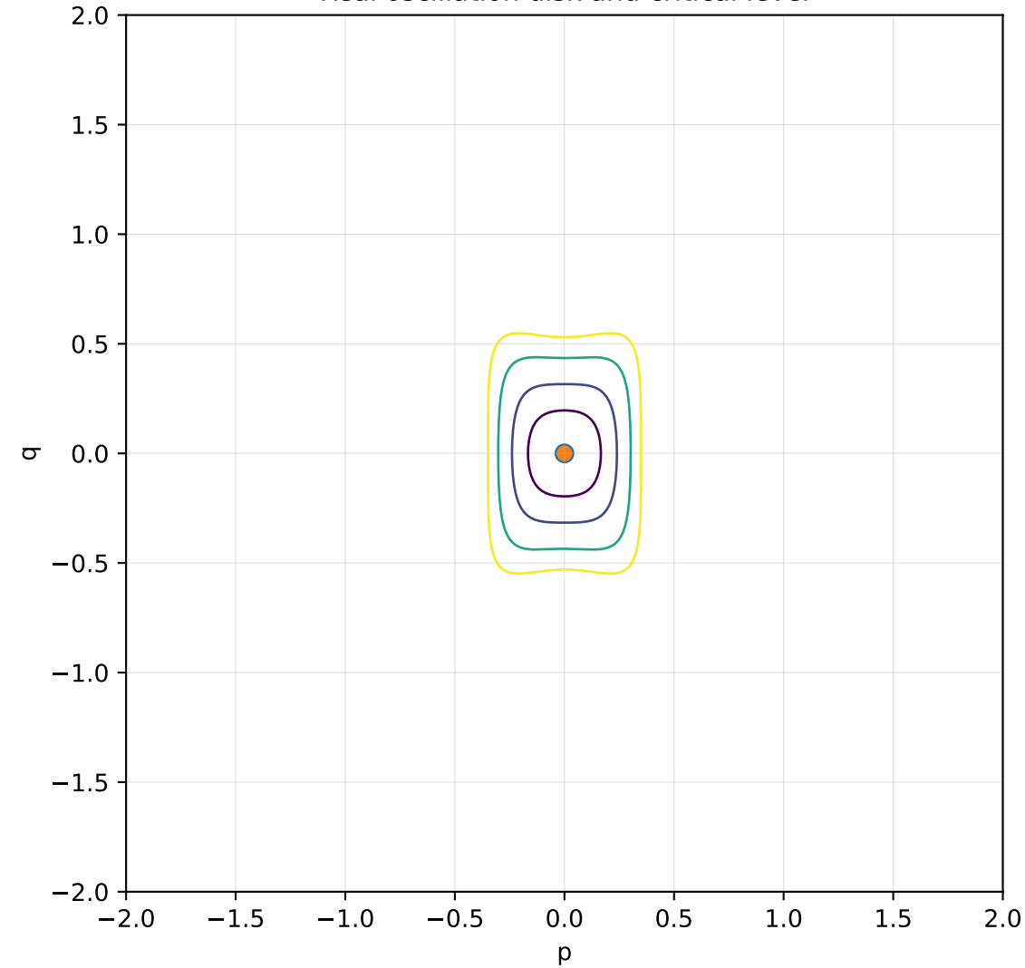
Real oscillation disk and critical level
