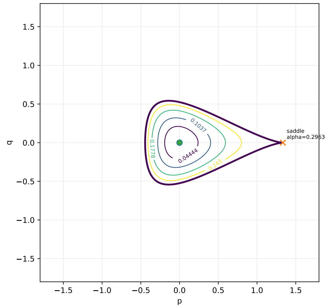
Real oscillation disk and critical level
