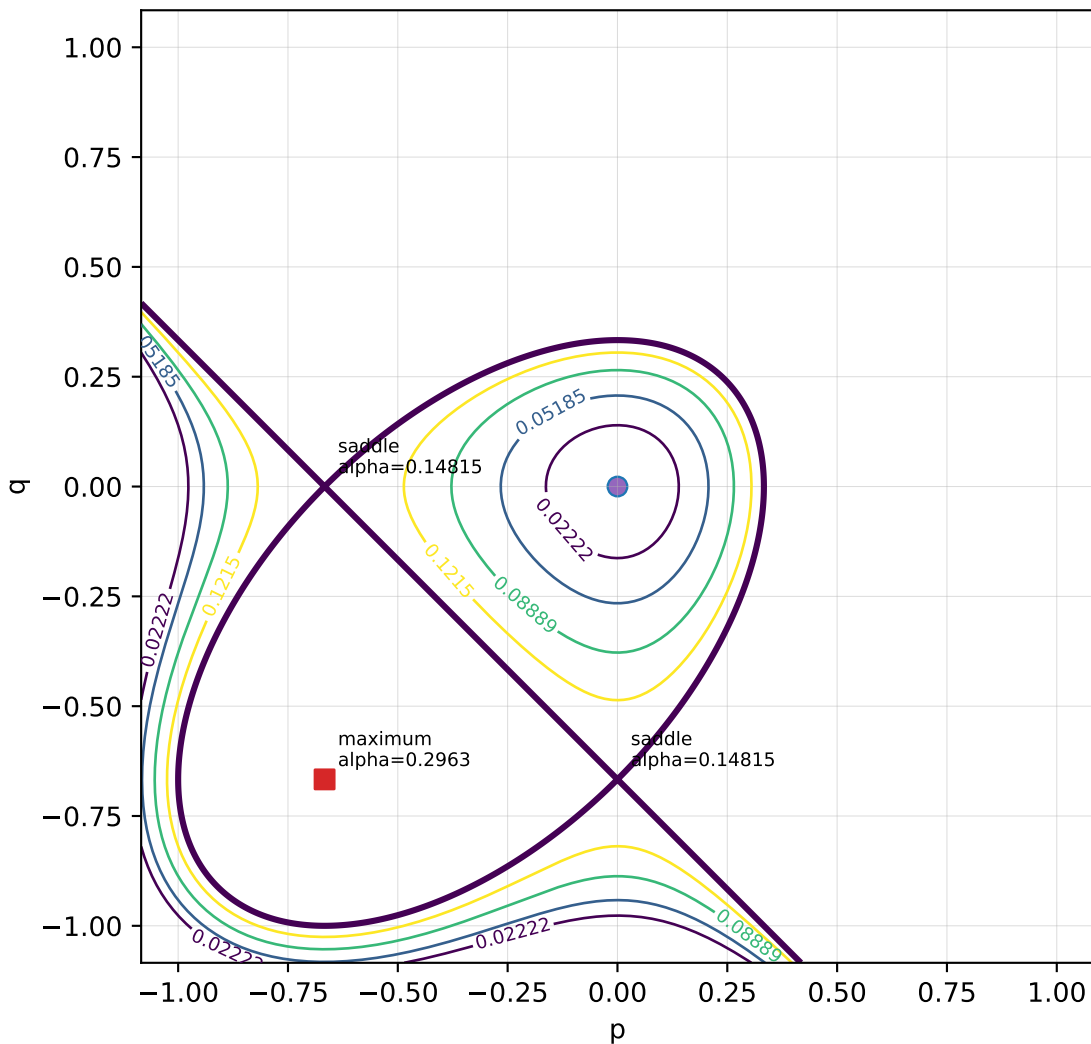
Real oscillation disk and critical level
