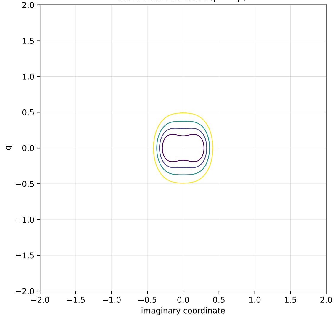
Abel-Wick real trace ( p \rightarrow ip )
