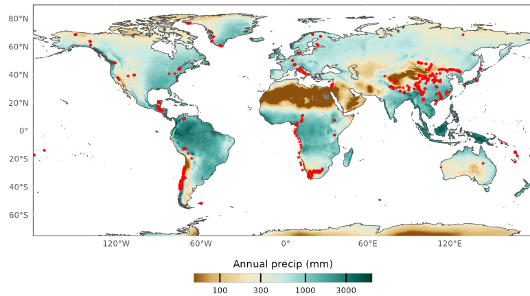
B: Annual precipitation
