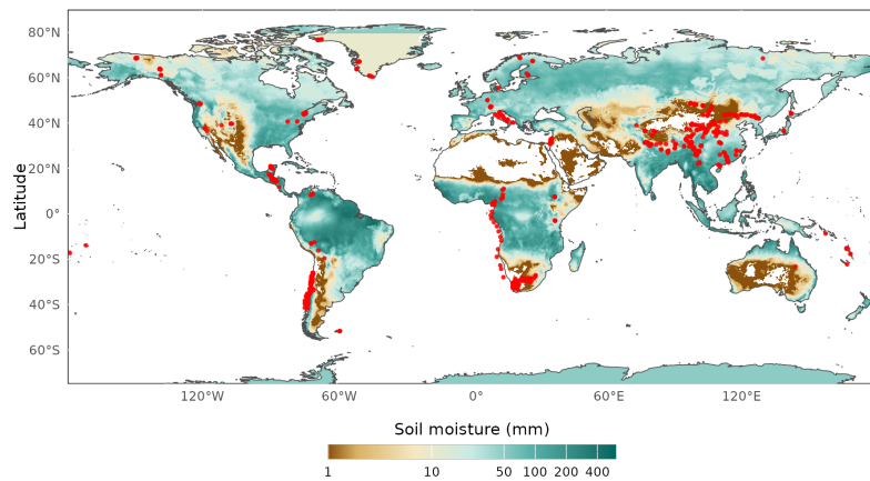
E: Soil moisture
