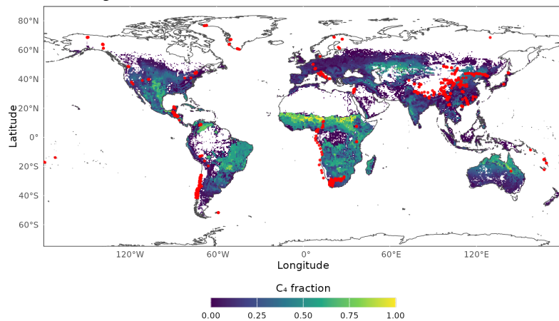
G: C 4 vegetation fraction
