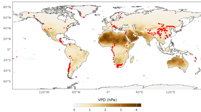
D: Vapor pressure deficit
