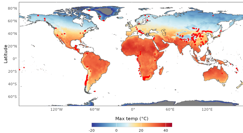
C: Maximum temperature
