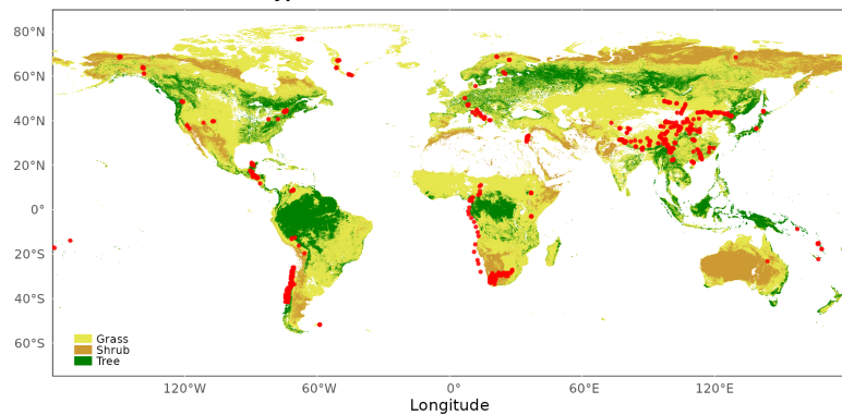
H: Plant Functional Type
