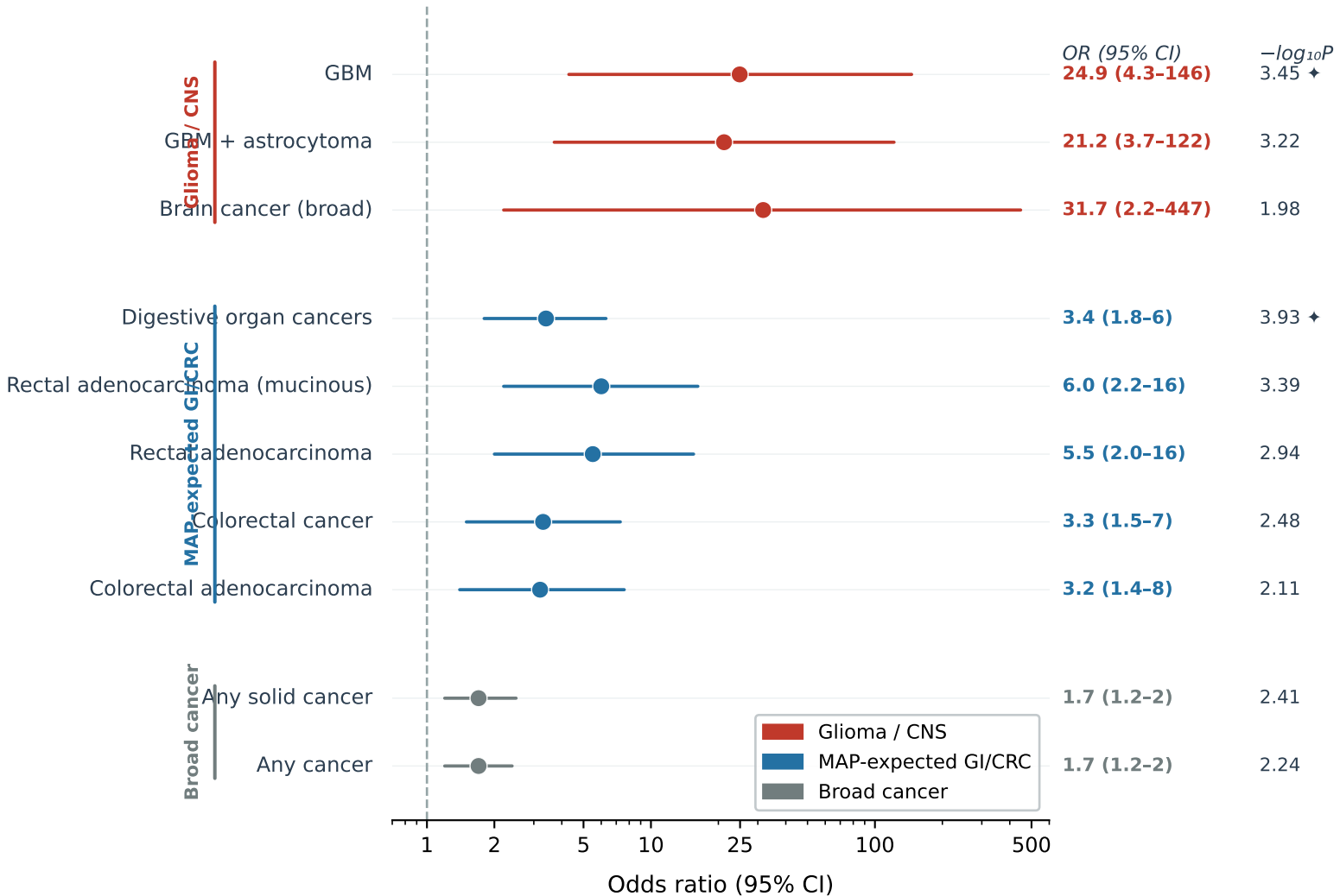
Supplementary Figure S1. FinnGen R13 phenotype-wide associations of MUTYH p.Gly155Asp (rs587781864) across cancer phenotypes
