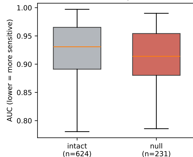
C Potent FAK-i PF-562271 — GDSC null more sensitive, p=9.7 \times 10^{-4}
