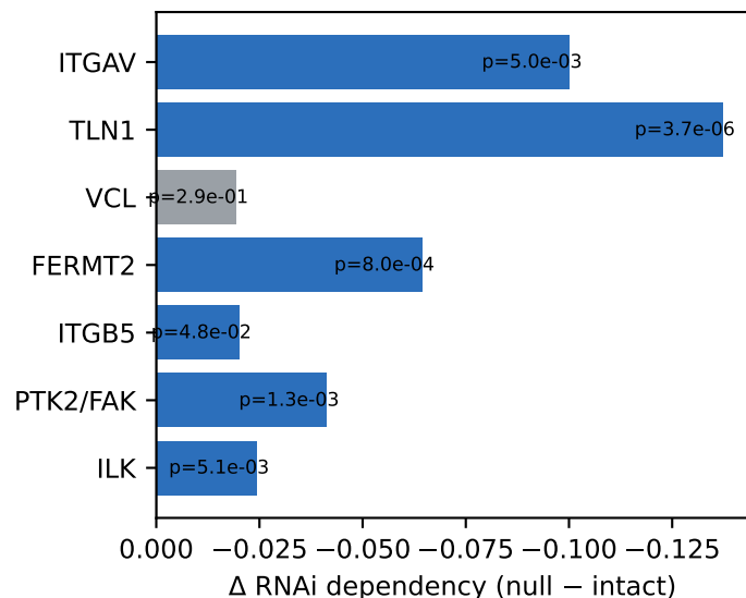
B RNAi shRNA — DEMETER2 (orthogonal) rules out CRISPR cut-artifact
