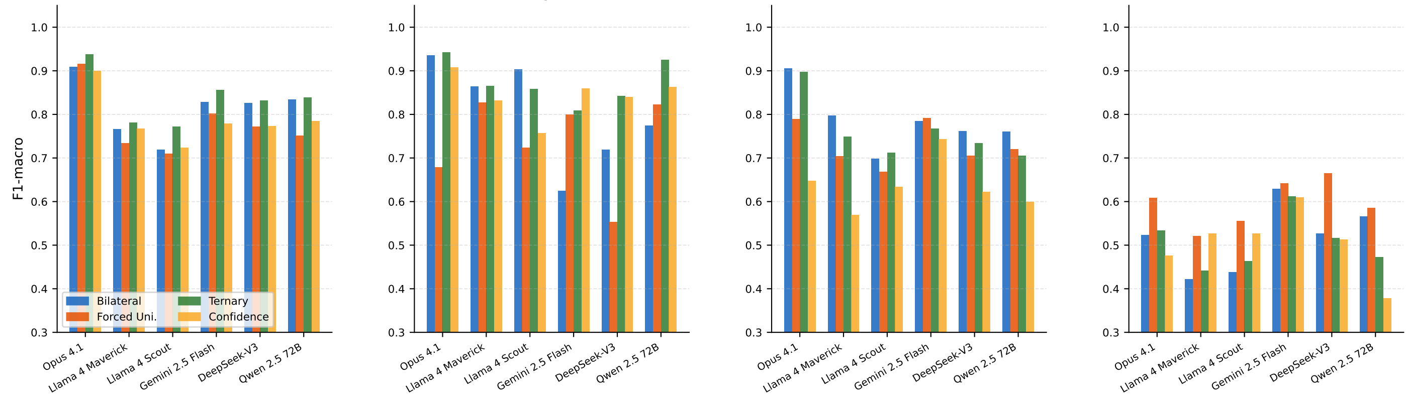
Panel A — F1-macro by Benchmark and Approach (N=250, bilateral N=3 majority vote, evidence-based ternary)
