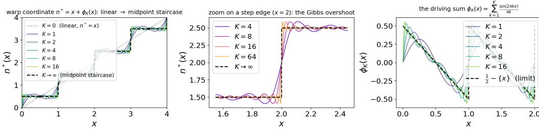
Figure 5: The warp coordinate n^*(x) = x + \varphi_K(x) bending from the linear x ( K = 0 ) into the midpoint staircase [x] + \frac{1}{2} as Fourier harmonics are restored. Panel (b): the \sim 9\% Gibbs overshoot at the step edges, which narrows but never vanishes, the source of the warp's non-elementary rate constant.
