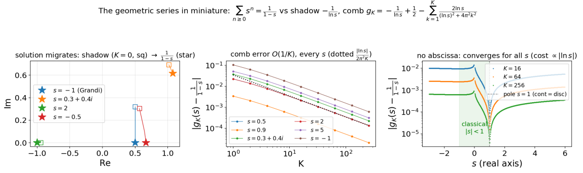
Figure 18: The geometric series in miniature ( geometric_bridge.py ). Left : with no zero string to move, the value g_K(s) migrates from the continuous shadow ( K = 0 , squares) onto the discrete sum 1/(1-s) (stars); at s = -1 it slides down \text{Re} = \frac{1}{2} from i/\pi to Grandi's \frac{1}{2} . Centre : the comb error is O(1/K) for every s , tracking |\ln s|/(2\pi^2 K) (31)—the arc's rate law with s \mapsto \ln s . Right : no abscissa—the error is smooth through the classical boundary |s| = 1 , dipping to 0 at the pole (shadow = sum) and growing like |\ln s| ; for |s| > 1 the interpolant sums the divergent series to 1/(1-s) .
