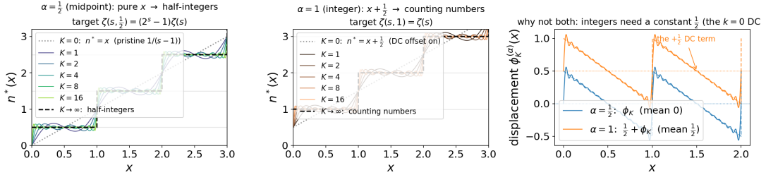
Figure 6: Two clean staircases: \alpha = \frac{1}{2} (half-integers) and \alpha = 1 (counting numbers). Panel (c) shows the obstruction: the \alpha = 1 displacement carries a constant DC term while \alpha = \frac{1}{2} does not. The half-integer midpoint is the unique clean staircase reachable from a pure- x start by pure trigonometric corrections, which is why it is the bridge's headline phase.
