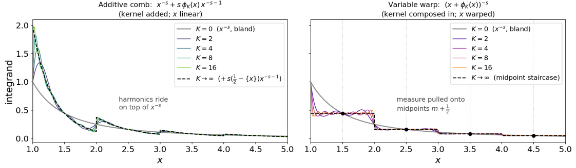
Figure 2: The two restoration routes drawn at the level of the integrand, at a real s = 2 and harmonic counts K = 2, 4, 8, 16 . Left : the additive comb x^{-s} + s\phi_K(x)x^{-s-1} (8) – the same kernel \phi_K is added on top of the smooth x^{-s} (grey, K = 0 ), an oscillation that converges to the full sawtooth ripple (dashed). Right : the variable warp (x + \phi_K(x))^{-s} (9) – the same kernel is composed into the argument , pulling the measure onto the cell midpoints m + \frac{1}{2} (dots) so the integrand collapses toward the midpoint staircase (dashed). Same kernel, same K , same K = 0 start; addition on the left, composition on the right.
