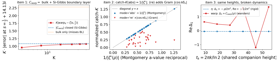
Figure 8: Three loose ends of the rate law: (i) a closed form for the warp constant C_{\text{warp}} as a Gibbs boundary-layer (sine-integral) integral; (ii) the tie of the birth threshold K_{\text{catch}} to the Montgomery a -values 1/|\zeta'(\rho)| ; and (iii) the fact that the \sigma = 1/\sigma = 0 companions share heights but not migration dynamics.
