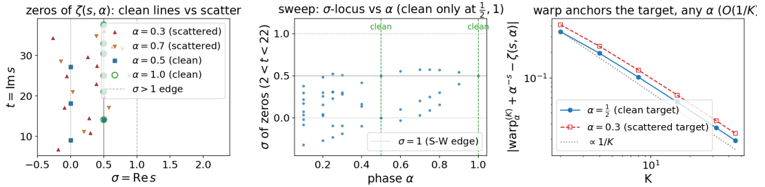
Figure 6: The general-phase n + \alpha warp onto \zeta(s, \alpha) , exhibiting the Saias–Weingartner dichotomy: clean vertical strings only at \alpha \in \{0, \frac{1}{2}, 1\} ; every generic \alpha is Davenport–Heilbronn scattered off-line. This locates the half-shift of Section 4 inside a one-parameter family and explains why \frac{1}{2} is special rather than merely chosen.
