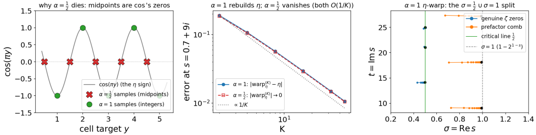
Figure 7: Warping the \eta integral (16). Left: the obstruction. The midpoints m + \frac{1}{2} that the \alpha = \frac{1}{2} warp samples are the zeros of the \eta sign-carrier \cos(\pi x) , while the integers m that \alpha = 1 samples sit on its extrema \pm 1 . Middle: consequently \alpha = 1 rebuilds \eta at O(1/K) while the \alpha = \frac{1}{2} warp vanishes. Right: the \alpha = 1 \eta -warp’s zeros migrate onto \sigma = \frac{1}{2} (genuine \zeta zeros) and \sigma = 1 (the prefactor comb): the same split as the additive comb (Fig. 3), by a second, independent route.
