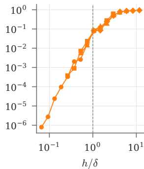
RMS ÷ the jump's
