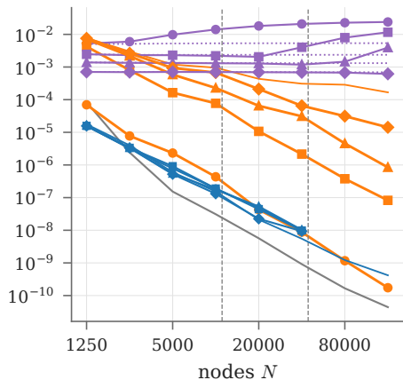
RMS ÷ the jump's
