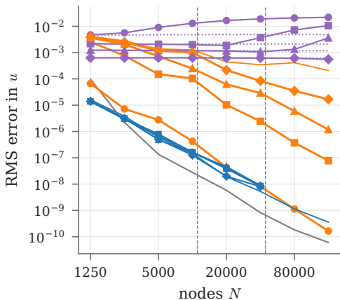
flux error, first pair
