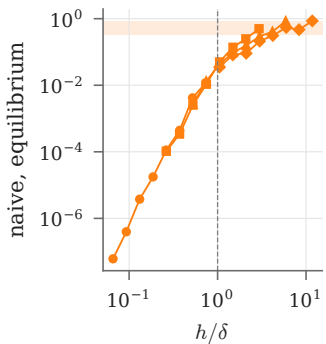
flux error, first pair
