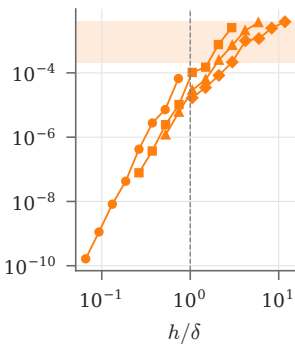
RMS error in u
