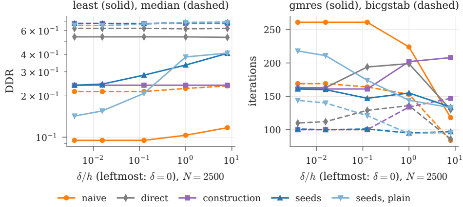
FIGURE 8. Case 1 at 2500 nodes against \delta/h (leftmost: the jump). Left: the least (solid) and median (dashed) diagonal dominance ratio over the seeded rows for the seeds and over the crossing rows for the other operators. Right: the iterations of GMRES (solid) and BiCGSTAB (dashed) without a preconditioner, to a relative residual of 10^{-8} . Seeds, plain: the seed rows with plain Gaussians.
