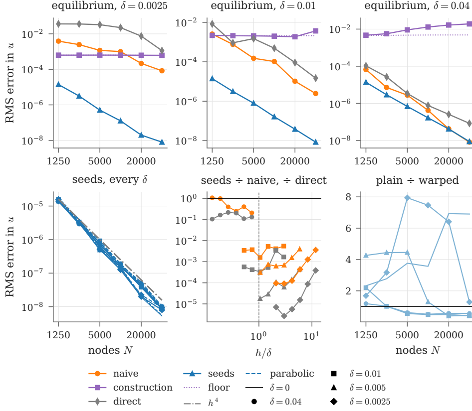
FIGURE 7. The seeds on case 1. Top: RMS error at equilibrium against the node count at \delta = 0.0025 , 0.01 and 0.04 , for the naive operator (orange), the \delta = 0 construction (purple) with its floor dotted, the direct operator (grey) and the seeds (blue). Bottom left: the seeds at every width, at equilibrium (solid) and for the parabolic problem (dashed); markers give \delta , the unmarked lines are the jump, and the dash-dotted line has the slope of h^4 . Bottom centre: the seeds' error over the naive operator's (orange) and the direct operator's (grey) against h/\delta . Bottom right: the seed rows with plain Gaussians over the warped ones (Table 20).
