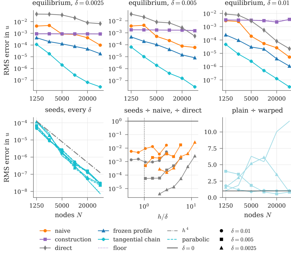
FIGURE 11. The tangential chain on case 2 (cyan), in the layout of Figure 7, with the frozen profile (blue) and the lines of Figure 10. Bottom: the tangential chain at every width, its ratios to the naive and direct operators against h/\delta , and plain over warped Gaussians.
