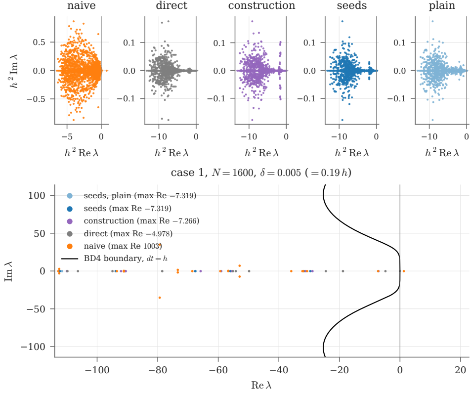
FIGURE 9. Interior eigenvalues \lambda on case 1 at 1600 nodes and \delta = 0.005 . Top: h^2\lambda for the naive operator, the direct operator, the \delta = 0 construction (construction), the seeds and the seeds with plain Gaussians (plain); the naive panel has its own axes, the others share theirs. Bottom: all five near the origin, with the boundary of BD4's region of absolute stability at \Delta t = h , left of which every mode is damped; the naive operator's rightmost eigenvalue lies off the panel.
