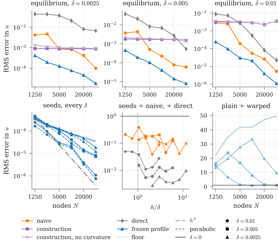
FIGURE 10. The straight-feature seeds with a frozen profile on case 2, in the layout of Figure 7. Top: RMS error at equilibrium against the node count at \delta = 0.0025, 0.005 and 0.01 , for the naive operator (orange), the \delta = 0 construction (purple), the same without its curvature terms (light purple), the direct operator (grey) and the frozen profile (blue). Bottom: the frozen profile at every width, its ratios to the naive and direct operators against h/\delta , and plain over warped Gaussians.
