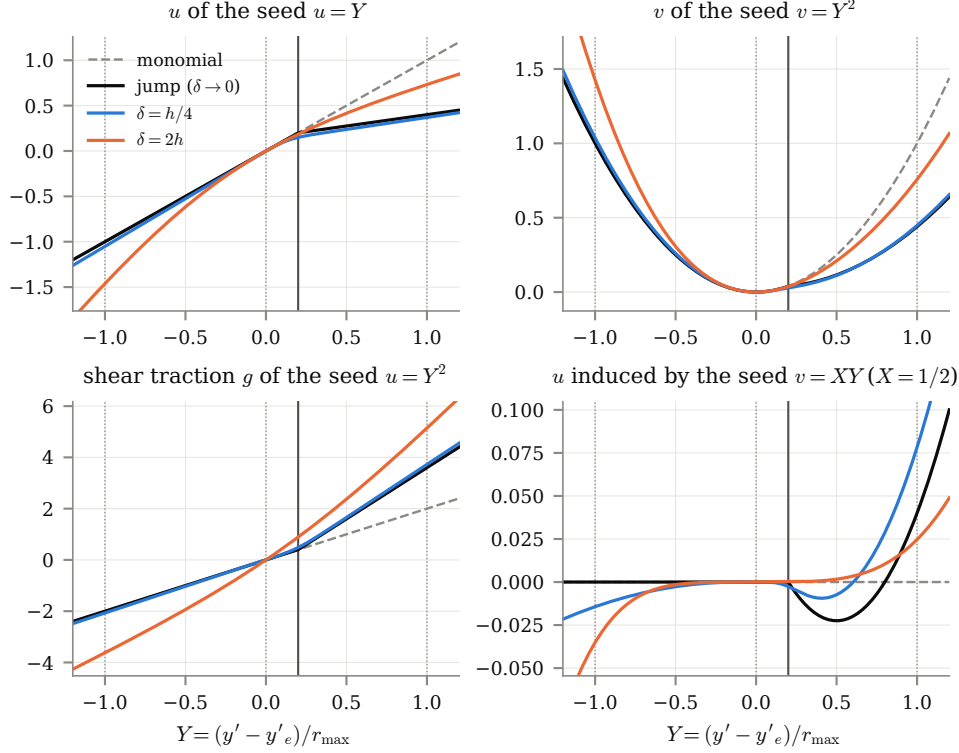
FIGURE 4. Cross-sections along the normal through the anchor of four elastic seeds of a 19-node stencil whose evaluation node lies h/2 below the lower edge of the band of Section 2.2 ( \lambda, \mu from 1 to 4, \rho from 1 to 2), in the stencil coordinate Y = (y - y_e)/r_{\max} with r_{\max} = 2.5h , for the jump limit (computed at \delta = 10^{-6} ), \delta = h/4 and \delta = 2h , against the monomials of the anchor material (dashed): the u of the seed u = Y ; the v of the seed v = Y^2 ; the shear traction of the seed u = Y^2 (labelled g , the implementation's name for the rate of \sigma_{xy} ); and the u induced by the seed v = XY at X = \frac{1}{2} , which is zero for the monomial and is the tangential coupling that the ablation of Section 6 removes. The vertical line is the edge centre and the dotted lines the stencil's reach |Y| \leq 1 . As in Figure 1, the \delta = h/4 seeds are close to the jump limit and the \delta = 2h seeds bend over the whole stencil.
