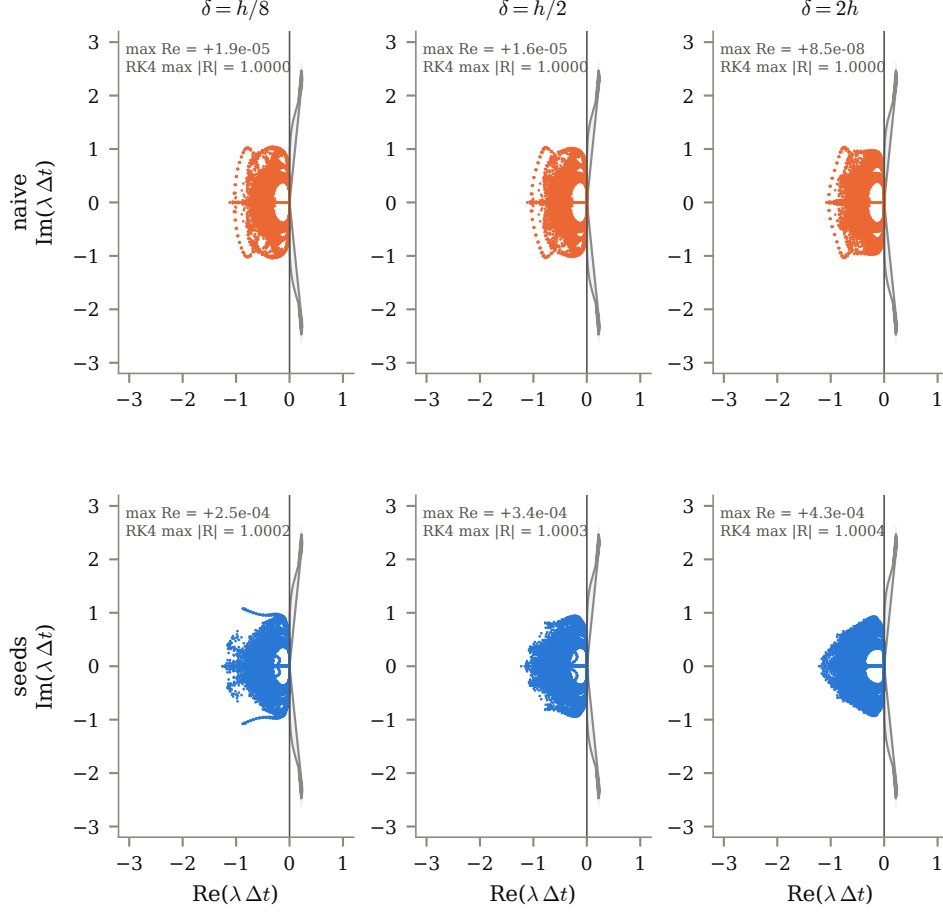
FIGURE 11. Spectra of the naive (top) and seed (bottom) operators on the 2500-node curved set through edges of width \delta = h/8, h/2 and 2h , as in Figure 5.
