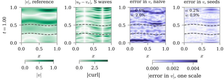
FIGURE 12. The pulse on 10,000 nodes through curved edges of width \delta = h/2 at t = 1 (the interfaces dashed): the reference |v| , its curl |u_y - v_x| (the S waves made at the curved edges), and the error in v of the naive scheme and of the seeds on one colour scale, with each map's relative errors in v and u .
