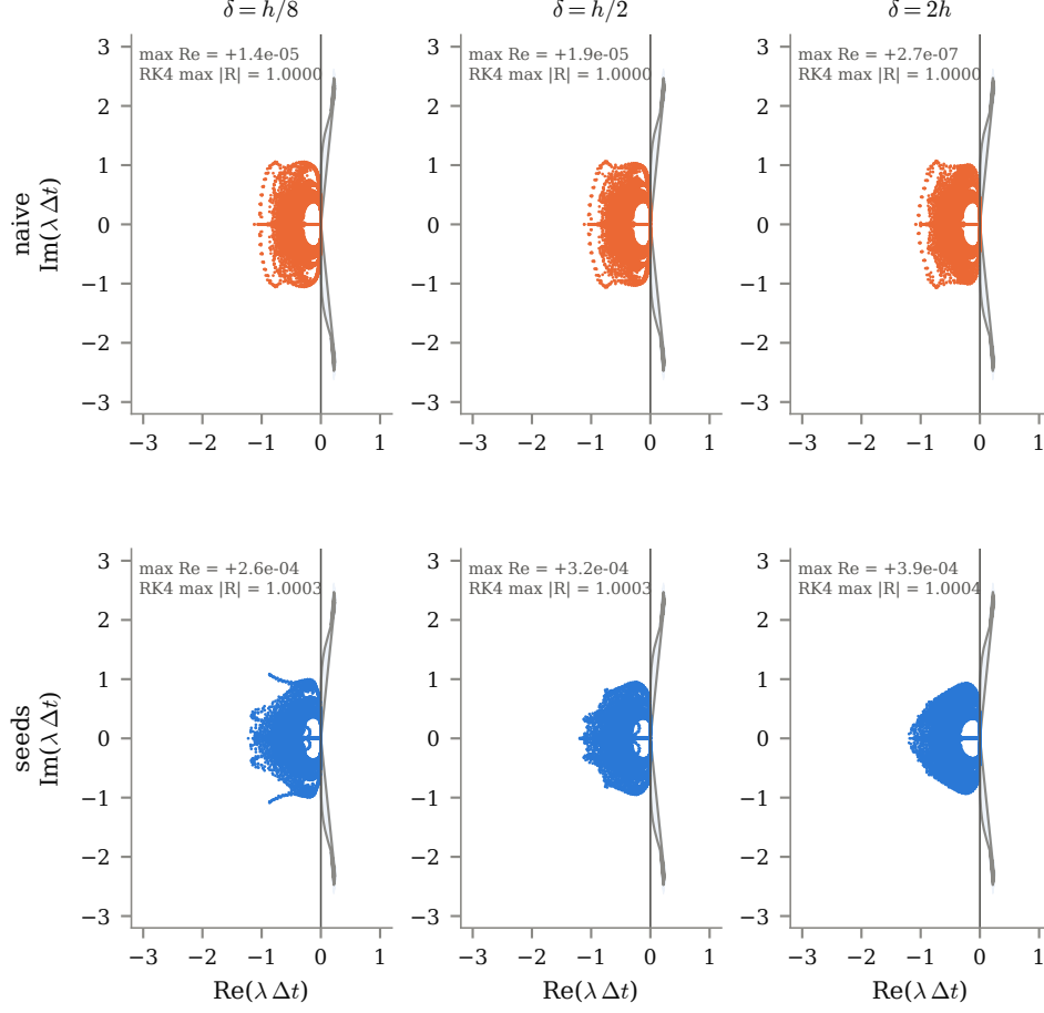
FIGURE 5. Spectra of the naive (top) and seed (bottom) operators on the 2500-node flat set through edges of width \delta = h/8 , h/2 and 2h , scaled by the time step, with the RK4 stability boundary. The annotations give the largest real part of \lambda \Delta t and the largest amplification over the spectrum.
