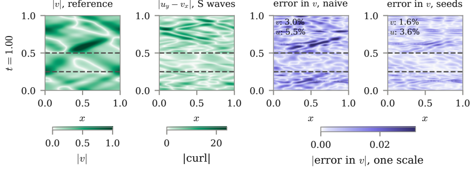
FIGURE 9. The train at 26.6^\circ on 10,000 nodes through flat edges of width \delta = h/4 at t = 1 : the reference |v| , its curl |u_y - v_x| (the mode-converted S waves), and the error in v of the naive scheme and of the seeds on one colour scale, with each map's relative errors in v and u .
