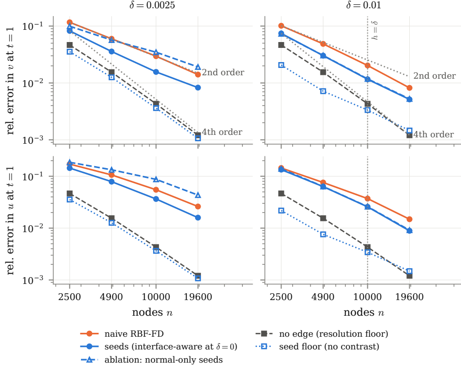
FIGURE 8. The oblique sweep of Tables 7 and 8: relative error in v (upper panels) and in u (lower panels) against n through \delta = 0.0025 and 0.01 , for the naive scheme, the seeds and the normal-only ablation, with the train's resolution floor and the seed floor. Every scheme converges at about second order through the sharp edge, and the ablation crosses above the naive scheme.
