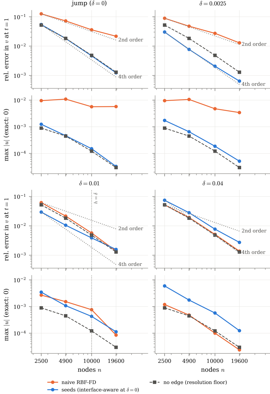
FIGURE 6. The flat sweep of Tables 2 and 3: relative error in v (upper panels) and largest spurious |u| (lower panels) against n for the jump and three edge widths, naive scheme against seeds, with the uniform-medium floor and second- and fourth-order guides; the vertical line in the \delta = 0.01 panel is the node set at which h = \delta . Through \delta = 0.0025 the seeds lie on a fourth-order line below the floor; through \delta = 0.04 they lie above the naive scheme, which is at the floor.
