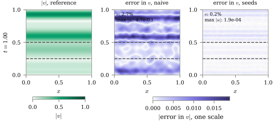
FIGURE 7. The pulse on 10,000 nodes through flat edges of width \delta = h/4 at t = 1 (the band between the dashed lines): the reference |v| , and the error in v of the naive scheme and of the seeds on one colour scale, with each map's relative error and largest spurious |u| .
