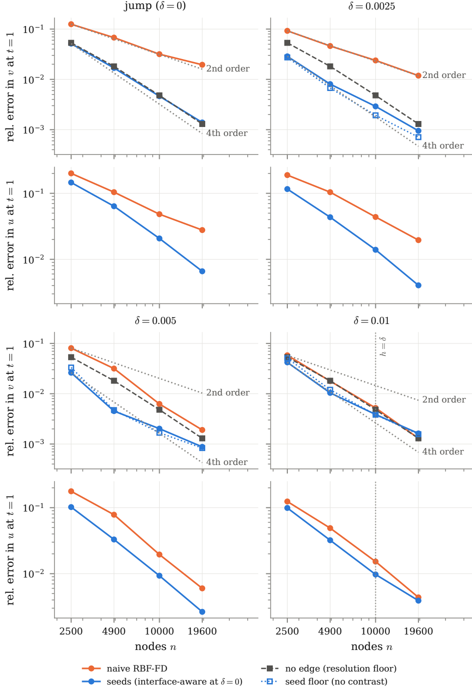
FIGURE 10. The curved sweep of Tables 10 and 11: relative error in v (upper panels) and in u (lower panels) against n for the jump and three edge widths, naive scheme against seeds, with the resolution floor and the seed floor; the vertical line in the \delta = 0.01 panel is the node set at which h = \delta . The jump stencils lie on the floor; through \delta = 0.0025 and 0.005 the seeds lie on the seed floor.
