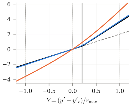
shear traction g of the seed u = Y^2
