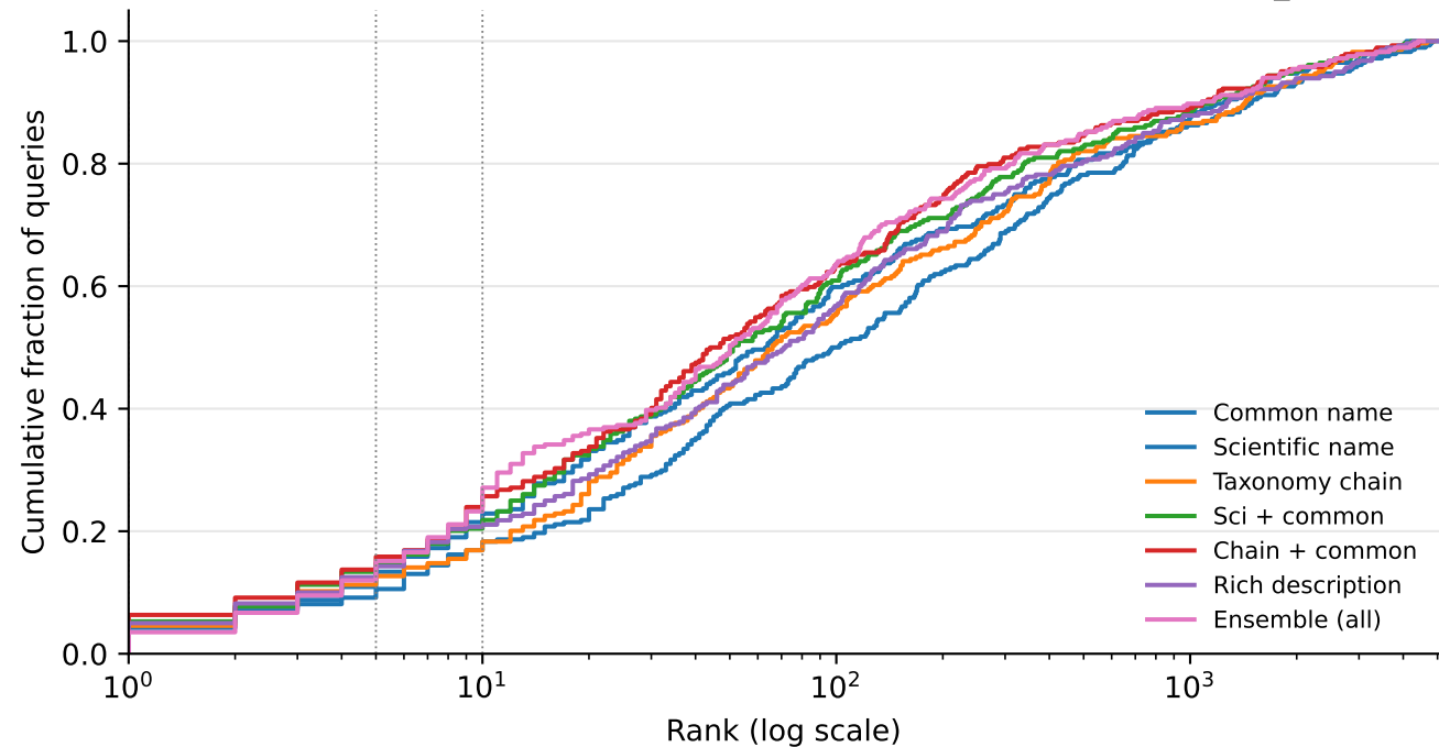
Rank CDF (fraction of queries with first hit \leq rank) — finetuned_zeroshot
