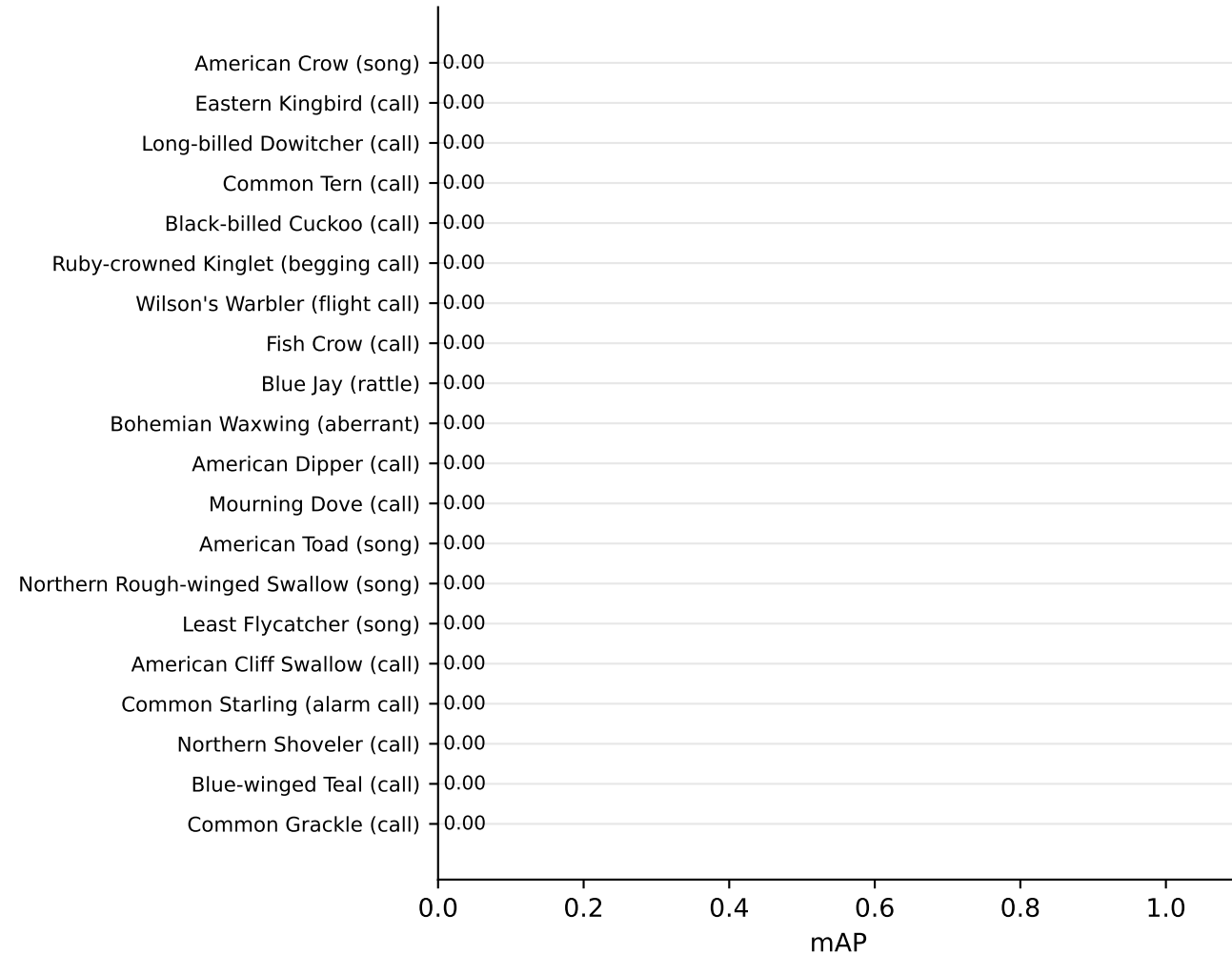
20 Hardest (lowest mAP)
