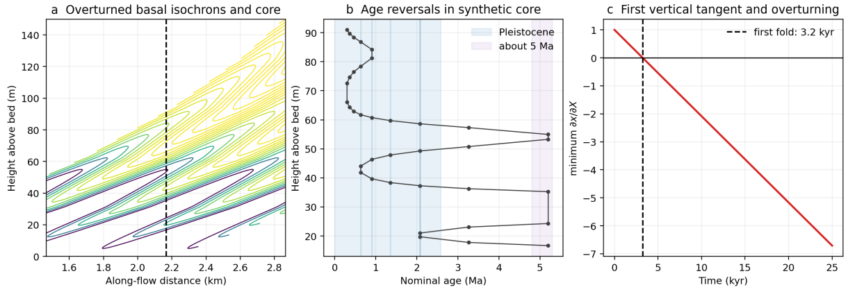
Figure 6: Overturned isochrons in the full-Stokes positive control. (a) The initially ordered isochrons after 25 kyr of advection through the n = 3 slab velocity field. The downstream-dipping limbs have rotated through vertical and become recumbent. The dashed line marks the synthetic core. (b) Repeated intersections of the overturned isochrons produce age reversals in the core. The nominal ages are schematic. (c) The minimum horizontal material derivative reaches zero after 3.2 kyr and is negative thereafter. This sign change, rather than layer relief alone, diagnoses overturning.
