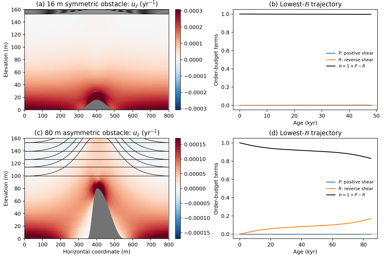
Figure 3: Full-Stokes order-budget examples. The left panels show vertical shear and five surface-origin trajectories for a low symmetric obstacle and a larger asymmetric obstacle. The right panels show the positive-shear contribution \mathcal{P} , reverse-shear expenditure \mathcal{R} and remaining order budget \mathcal{B} for the trajectory with the lowest final budget in each case. Local reverse shear is appreciable for the asymmetric obstacle, but \mathcal{B} remains positive.
