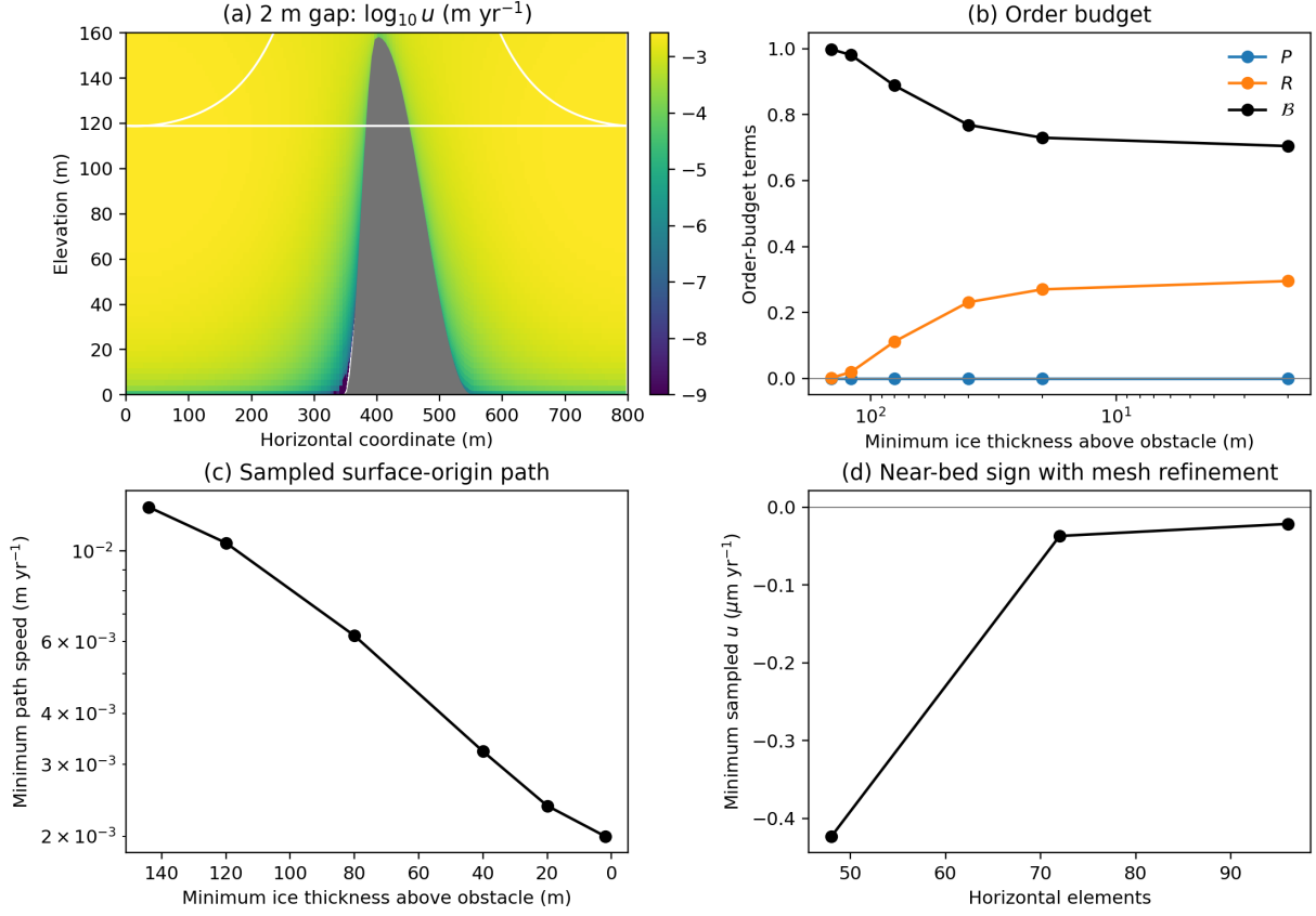
Figure 5: Approach to near-stagnation. (a) Horizontal speed and the sampled surface-origin trajectory for a 2 m gap. (b) Positive shear, reverse shear and the order budget as the gap narrows. (c) Minimum horizontal speed along the surface-origin trajectory. (d) Minimum near-bed velocity sampled on three meshes. The negative values approach zero with refinement and do not establish a resolved flow reversal.
