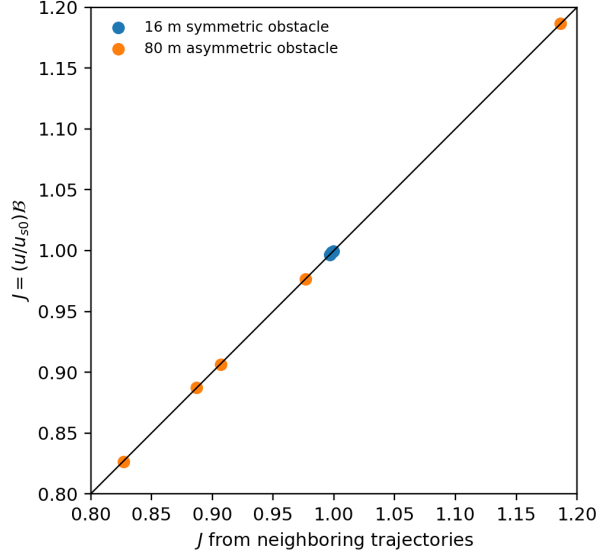
Figure 4: Independent evaluation of the order Jacobian. The horizontal axis uses equal-age trajectories initialized at x_0 \pm 0.05 m; the vertical axis uses Equation (27). The line shows equality.
