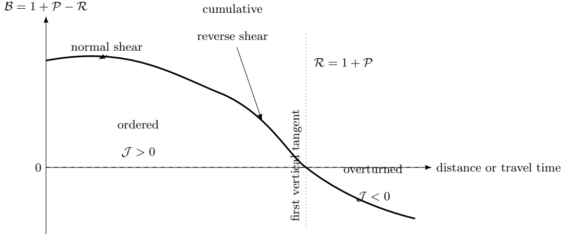
Figure 2. Conceptual order budget. The sign of \mathcal{B} = 1 + \mathcal{P} - \mathcal{R} is the sign of the order Jacobian. Local reverse shear need not cause overturning; a vertical tangent appears only after cumulative reverse shear removes the initial depositional contribution and the accumulated normal-shear contribution.
