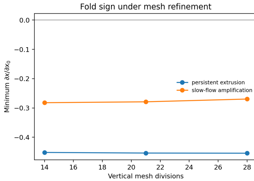
Figure 5. Mesh check for the boundary-generated folds. The ordinate is the minimum value of \partial x / \partial x_0|_{\tau} evaluated from neighboring surface-origin trajectories at 2.5 kyr and 0.8 kyr for the persistent-extrusion and slow-flow examples, respectively. Both calculations retain a negative interval on the three meshes.
