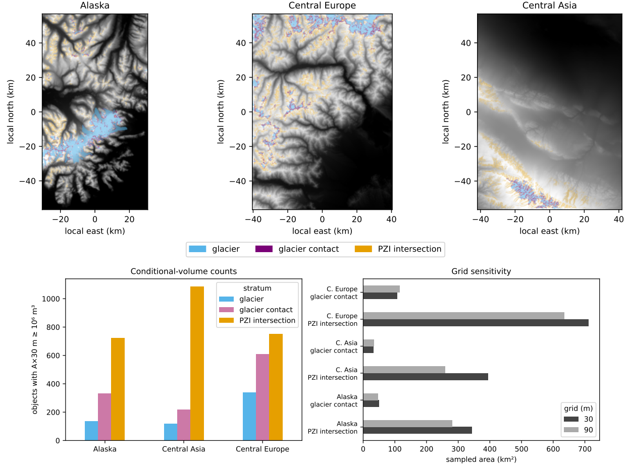
Figure 1: Climate- and case-blind susceptible-terrain pilot. Top: the three deterministically selected windows with RGI glacier polygons, primary steep glacier-contact terrain, and primary steep PZI-intersection terrain. Bottom left: object counts meeting the conditional V = A(30 \text{ m}) threshold. Bottom right: primary rock-slope area at 30 and 90 m. Strata overlap, source epochs differ, and none of the mapped objects is a predicted failure. Elevation products were produced using Copernicus WorldDEM-30 © DLR e.V. 2010–2014 and © Airbus Defence and Space GmbH 2014–2018, provided under COPERNICUS by the European Union and ESA; all rights reserved.
