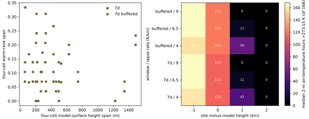
Figure 3: Registered topographic sensitivity. The left panel compares the four-cell model-surface-height range with the corresponding warm-state-rank range for both seven-day windows. The right panel gives the median number of 2-m air-temperature hours above 273.15 K for every window, lapse-rate, and site-minus-model-height scenario. It does not diagnose material thaw, and the scenarios are not estimates of source elevation.
