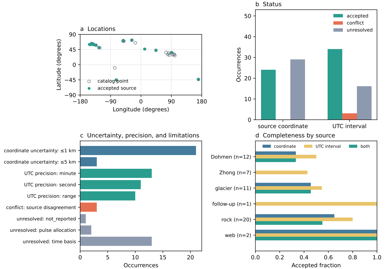
Figure 1: Climate-blind source-coordinate and UTC-onset audit. (a) The 29 finite original catalog points and 24 accepted source coordinates. (b) Accepted, conflicting, and unresolved outcomes. (c) Accepted coordinate uncertainty, accepted UTC precision, and reasons for non-accepted times. (d) Acceptance fractions by discovery stream. Nine accepted UTC intervals are earthquake trigger-origin proxies, not detachment clocks. The figure contains no climate or reanalysis values.
