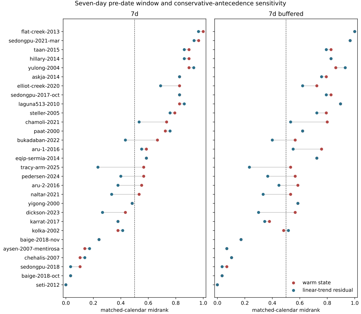
Figure 1: Registered seven-day ERA5 temperature ranks for the pre-date window (left) and conservative-antecedence sensitivity (right), using a common occurrence order. Red points rank event-year means against matching 1991–2020 calendar windows; blue points apply the same rank after removing a robust 1979–2025 linear trend. Lines join two diagnostics for one occurrence. The dashed line at 0.5 is a reference median, not a fitted failure threshold.
