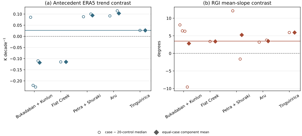
Figure 14: Matched contrasts for (a) strictly antecedent 20-year ERA5 2-m air temperature trends and (b) mixed-epoch RGI 7 glacier-wide mean surface-slope attributes. Open points are documented cases minus the median of their 20 frozen matched RGI comparison objects; filled diamonds are equal-case means within final dependence components. Components receive equal weight. Solid lines mark median component contrasts and dashed lines mark zero. ERA5 is a regional atmospheric exposure at model orography; RGI slope does not measure pre-event source geometry. Neither panel establishes a warming-trigger mechanism, failure probability, risk, or causation.
