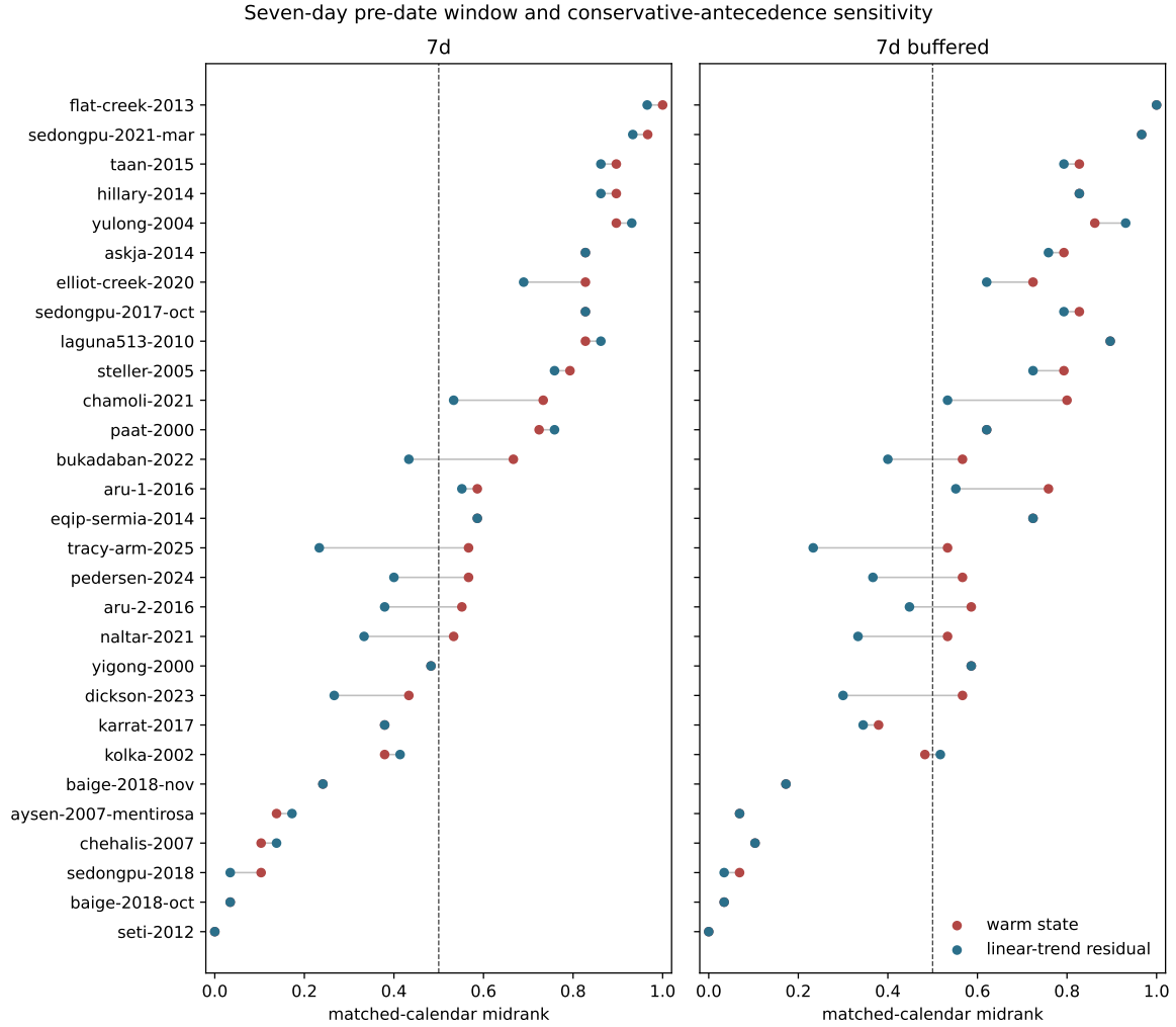
Figure 9: Registered seven-day ERA5 temperature ranks for the pre-date window (left) and conservative-antecedence sensitivity (right), using a common occurrence order. Red points rank event-year means against matching 1991–2020 calendar windows; blue points apply the same rank after removing a robust 1979–2025 linear trend. Lines join two diagnostics for one occurrence. The dashed line at 0.5 is a reference median, not a fitted failure threshold.
