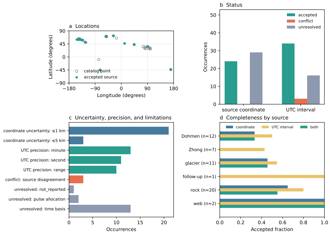
Figure 8: Climate-blind source-coordinate and UTC-onset audit. (a) The 29 finite original catalog points and 24 accepted source coordinates. (b) Accepted, conflicting, and unresolved outcomes. (c) Accepted coordinate uncertainty, accepted UTC precision, and reasons for non-accepted times. (d) Acceptance fractions by discovery stream. Nine accepted UTC intervals are earthquake trigger-origin proxies, not detachment clocks. The figure contains no climate or reanalysis values.
