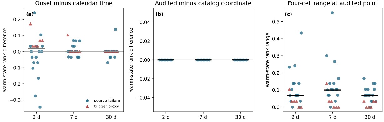
Figure 13: Source-verified ERA5 assignment sensitivity. (a) Primary-cell warm-state-rank change from catalog-date midnight to the audited onset endpoint for all 22 occurrences. (b) Primary-cell rank change from catalog to audited coordinates for the nine old-pilot overlaps. Each retained the same primary grid cell. (c) Rank range among the four cells bracketing each nominal audited coordinate. Circles are measured source-failure intervals; triangles are event-specific earthquake trigger proxies. Black bars are medians, not decision thresholds. The four-cell range does not propagate positional uncertainty.
