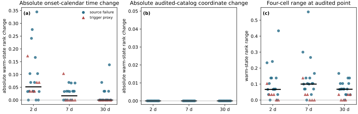
Figure 13: Source-verified ERA5 assignment sensitivity. (a) Absolute primary-cell warm-state-rank change from catalog-date midnight to the audited onset endpoint for all 22 occurrences. (b) Absolute primary-cell rank change from catalog to audited coordinates for the nine old-pilot overlaps. Each retained the same primary grid cell. (c) Rank range among the four cells bracketing each nominal audited coordinate. Circles are measured source-failure intervals; triangles are event-specific earthquake trigger proxies. Black bars are medians, not decision thresholds. The four-cell range does not propagate positional uncertainty.
