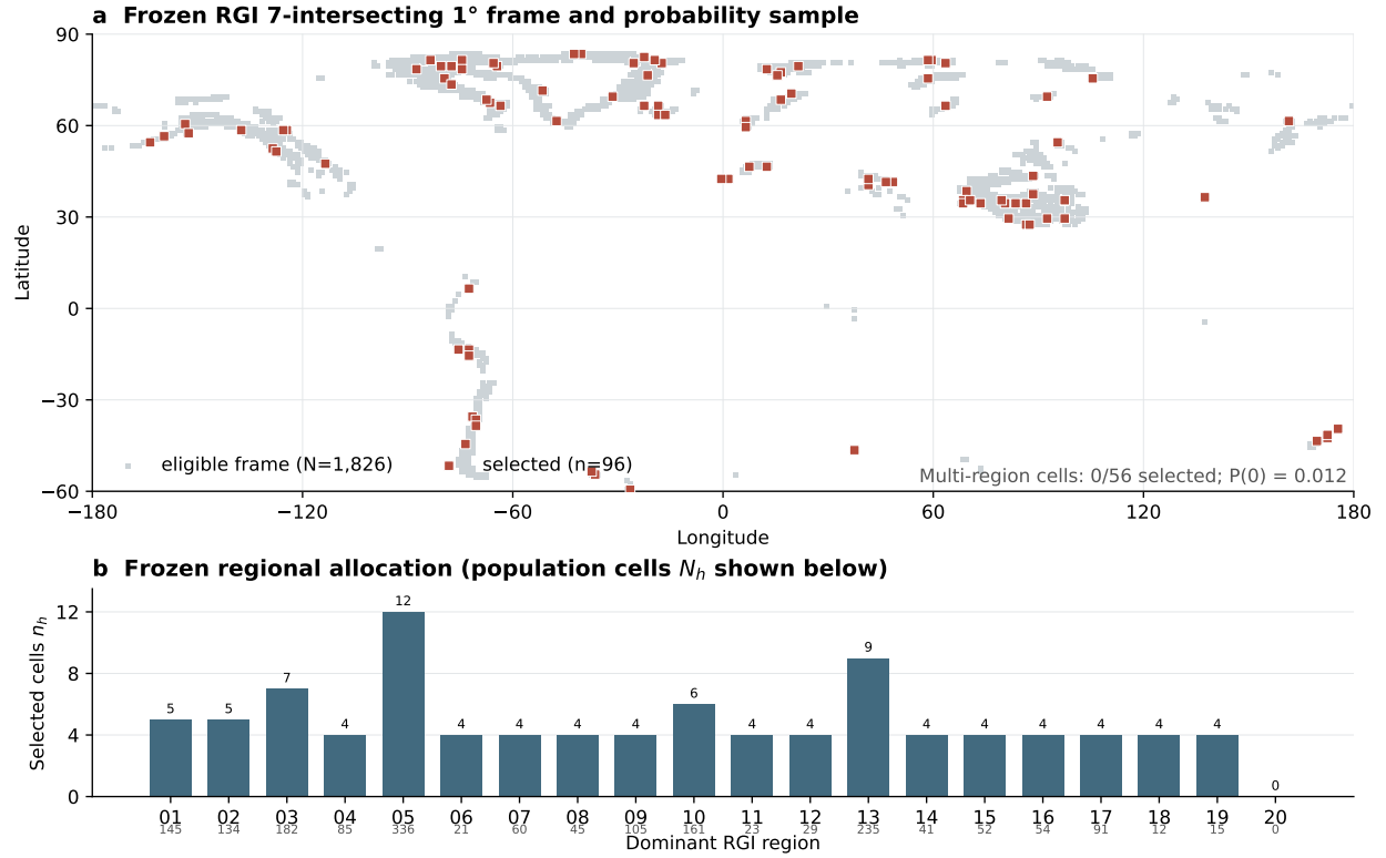
Figure 5: Frozen geographic probability frame and signed-beacon draw. (a) Centers of all 1,826 eligible 1° cells and the 96 selected cells. The probability of selecting none of the 56 multi-region cells is a post-randomization balance diagnostic under the frozen design; no redraw was made. (b) Selected count in each of 19 nonempty dominant-region strata; population counts appear below the region codes. Empty RGI region 20 is shown with N_{20} = n_{20} = 0 . The figure describes sampling support only; no DEM, PZI, climate, event, or terrain-outcome value entered the frame or draw.
