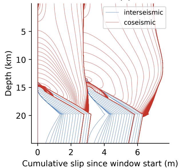
S3d Cumulative slip profiles
