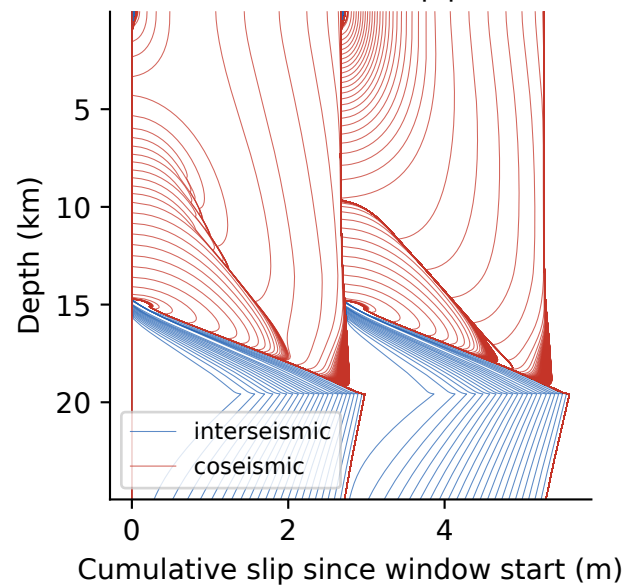
S3b Cumulative slip profiles
