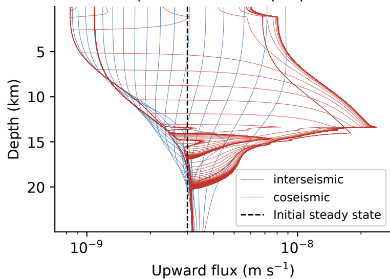
S4f Upward fluid flux depth profiles
