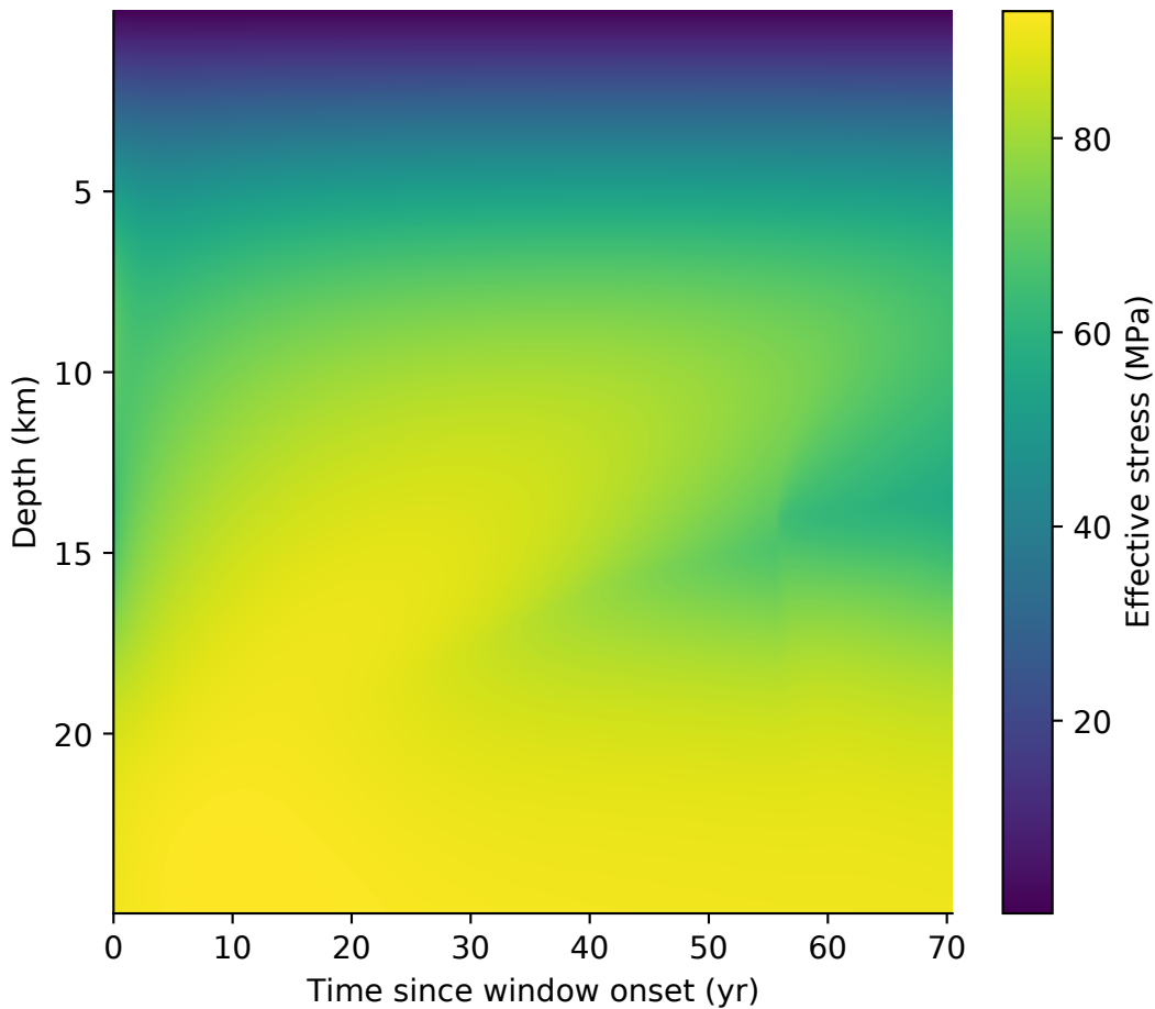
S4a Effective normal stress history
