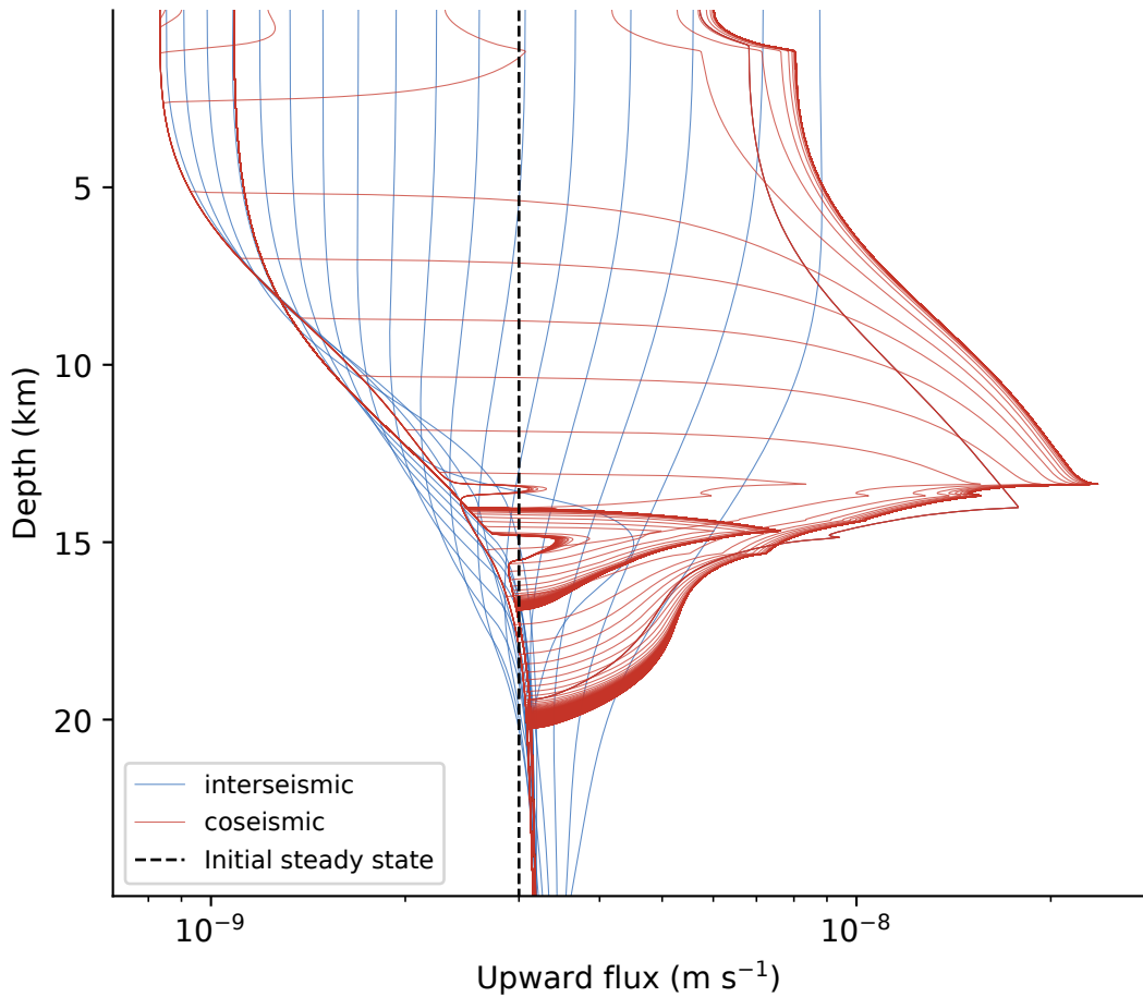
S4f Upward fluid flux depth profiles
