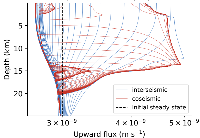
S6f Upward fluid flux depth profiles
