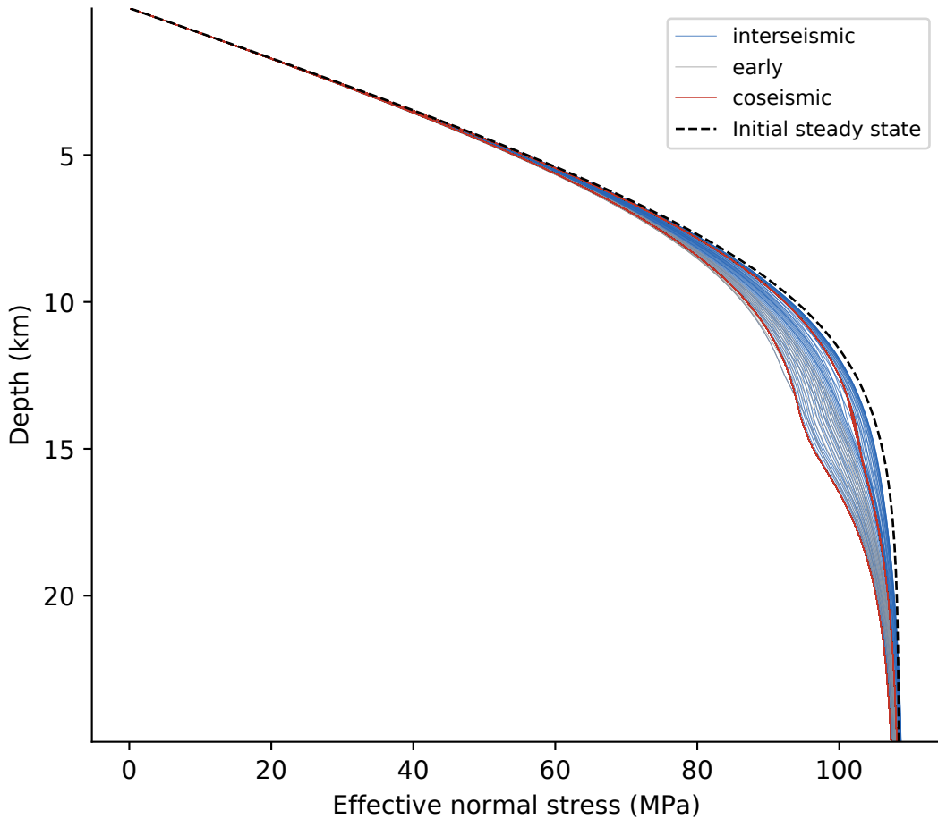
S6b Effective normal stress depth profiles
