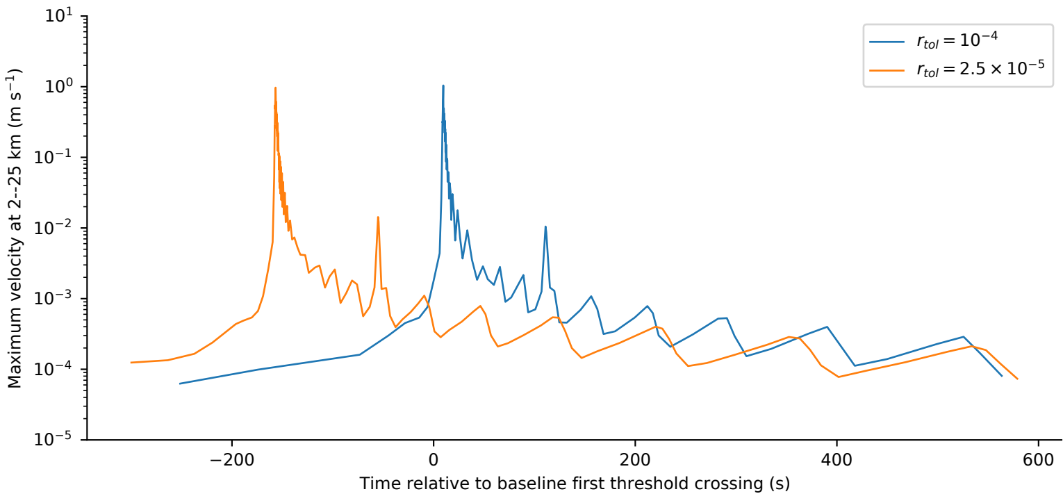
First seismic event: identical initial checkpoint, two time tolerances
