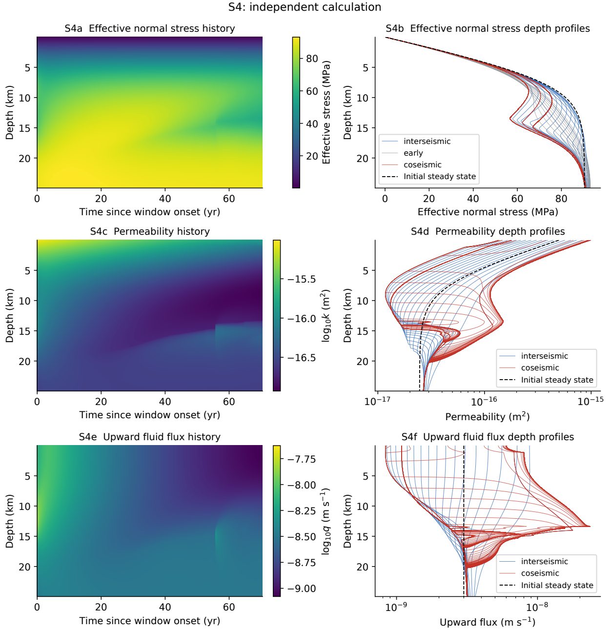
Figure 10: Independent outputs corresponding to S4. S4a: Effective normal stress history; S4b: Effective normal stress depth profiles; S4c: Permeability history; S4d: Permeability depth profiles; S4e: Upward fluid flux history; S4f: Upward fluid flux depth profiles. Units and color scales are shown on the panels. Parameter files and selection rules are specified in the provenance sidecars. Cases: long ( T=1\text{e}+09 s; coupled pressure). These panels are partial comparisons. Comparison target: Zhu et al. [1].
