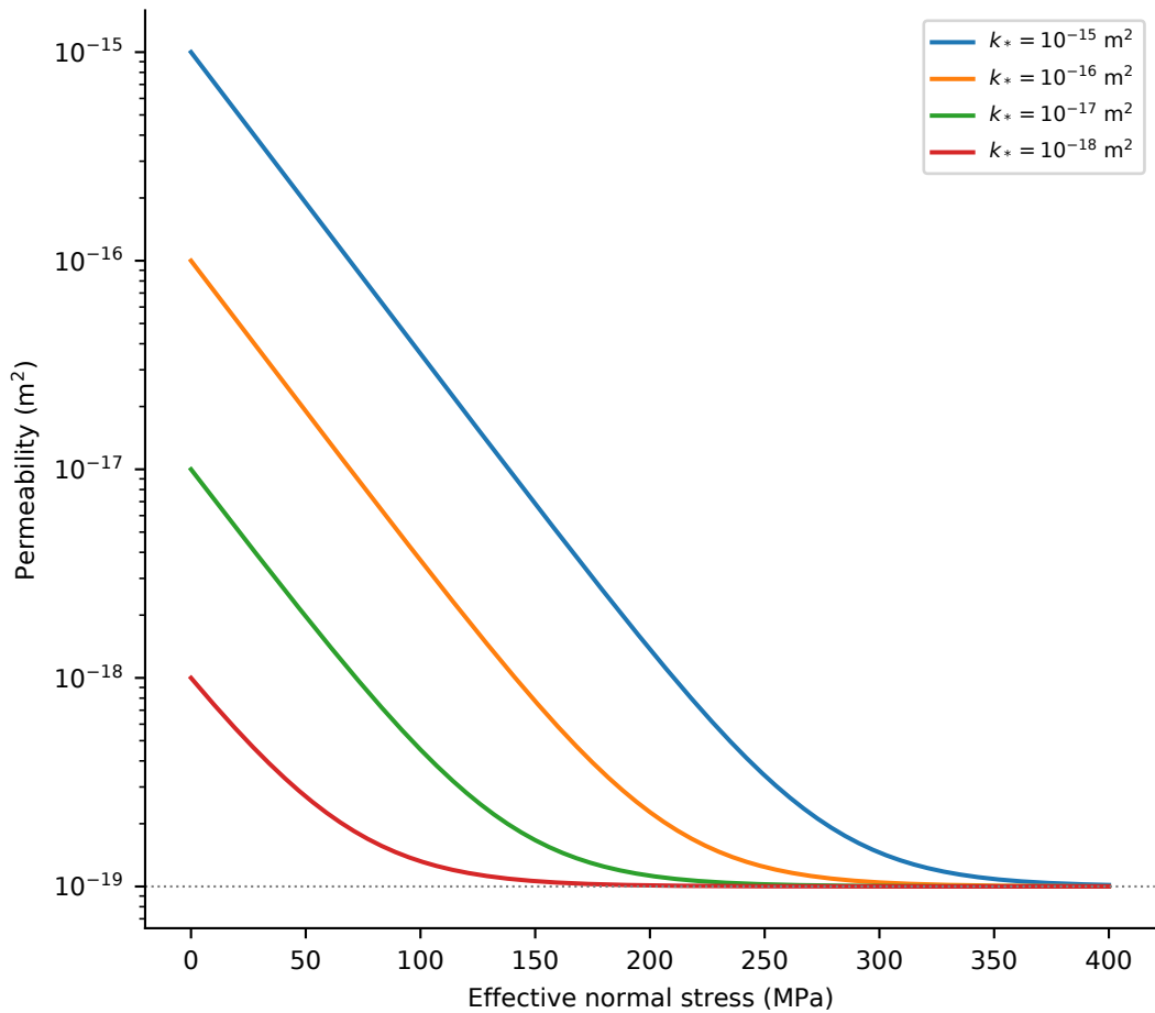
F1b Permeability versus effective normal stress
