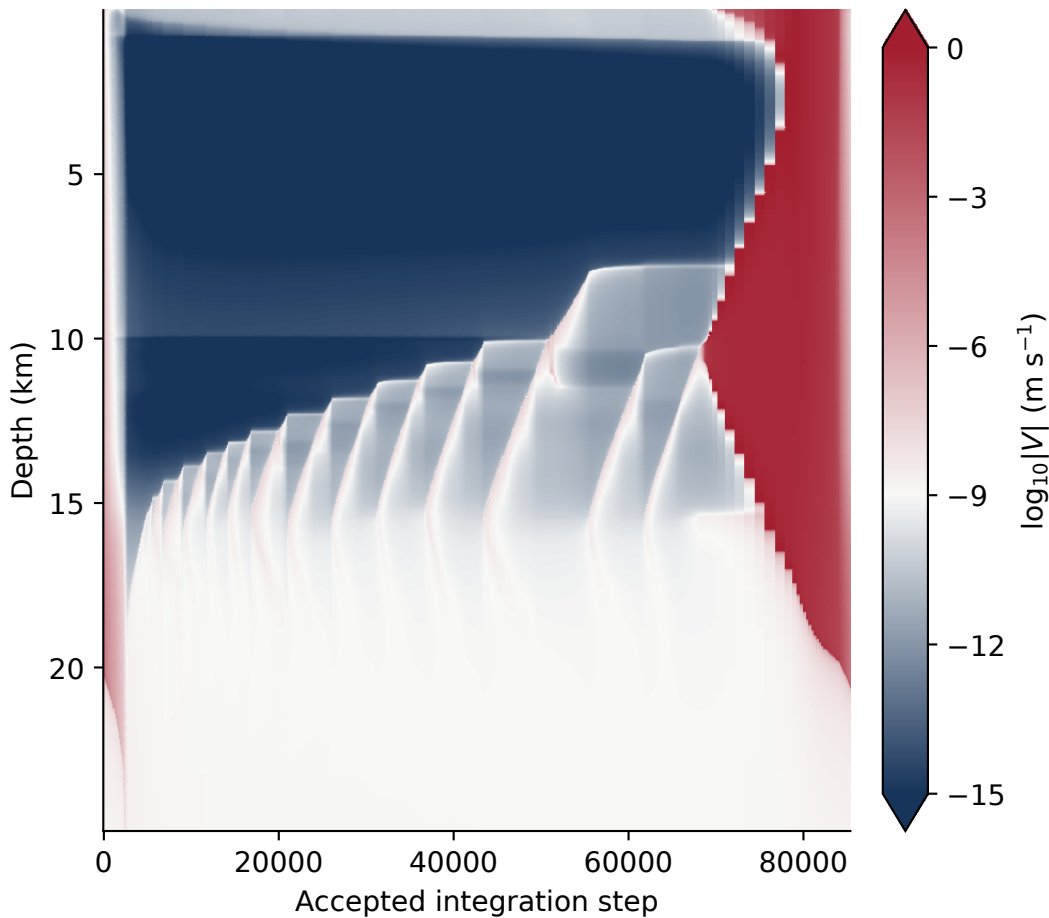
F5b Slip velocity versus accepted step
