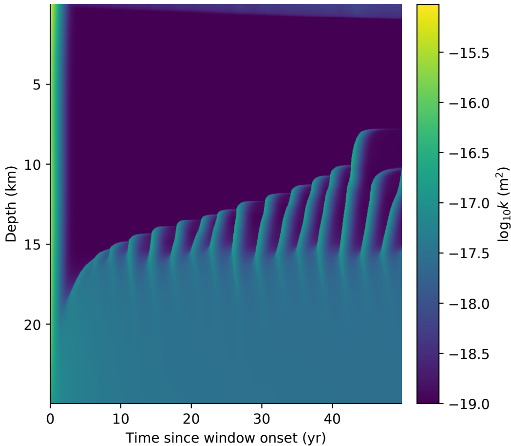
F5d Permeability
