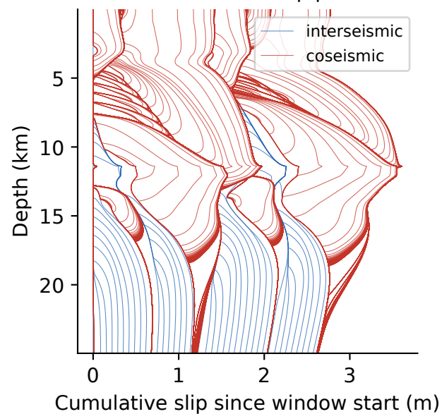
F2d Cumulative slip profiles
