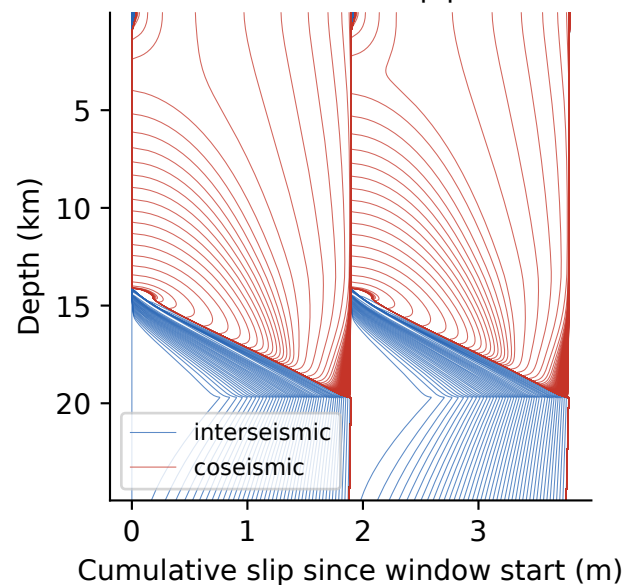
F2b Cumulative slip profiles
